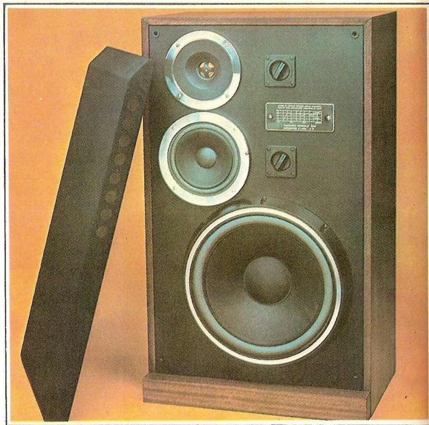
ZG 80C 11
