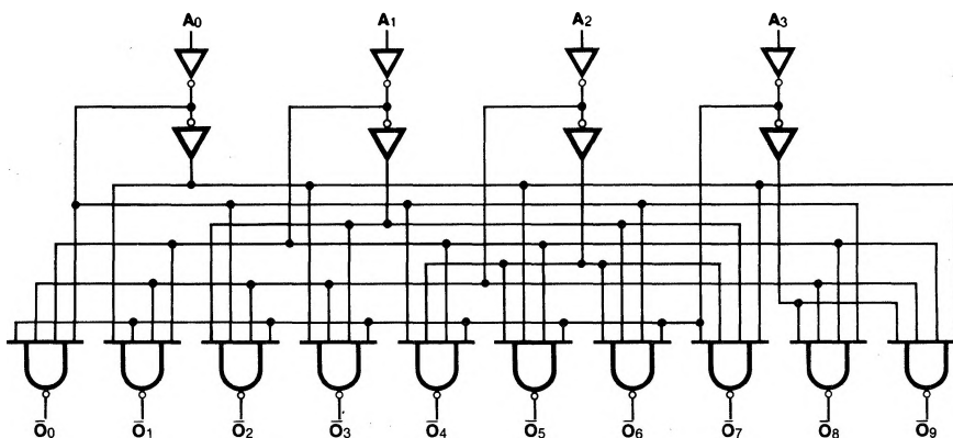
LOGIC DIAGRAM
