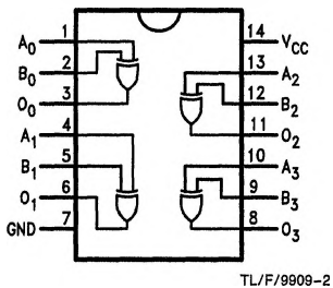
Pin Assignment for DIP, Flatpak and SOIC
