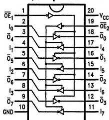
Pin Assignment for DIP, Flatpak and SOIC
