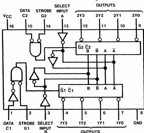
Dual-In-Line Package
