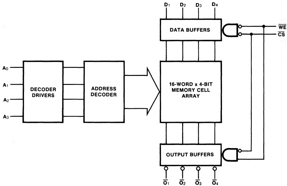
LOGIC DIAGRAM
