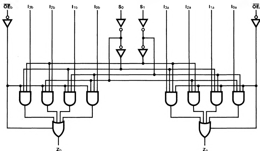
LOGIC DIAGRAM
