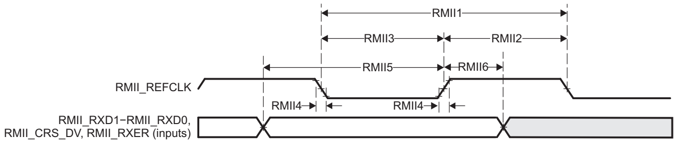
Figure 5-30. EMAC Receive Interface Timing RMI operation
