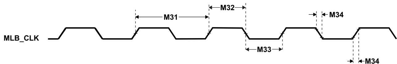
Figure 5-53. MLB_CLK Timing
