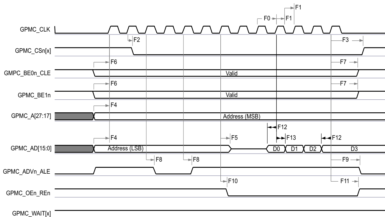
Figure 5-39. GPMC and Multiplexed NOR Flash—Synchronous Burst Read
