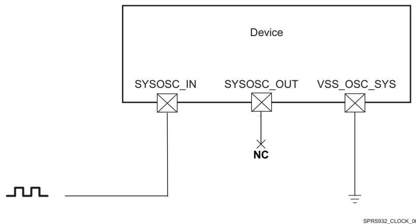
Figure 5-11. LVCMOS-Compatible Clock Input
