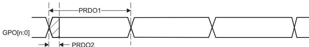
Figure 5-63. PRU-ICSS PRU Direct Output Timing
