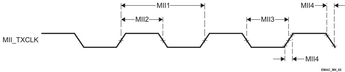
Figure 5-27. Clock Timing (EMAC Transmit)—MII operation
