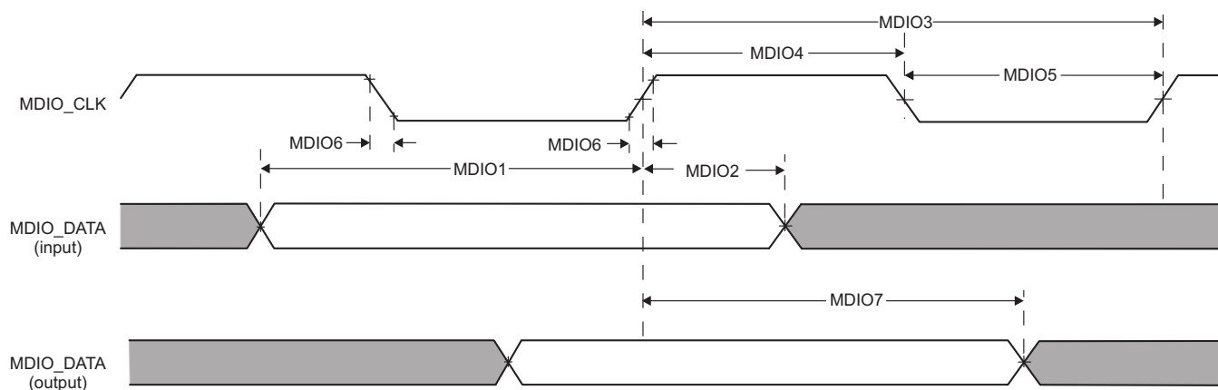
Figure 5-25. EMAC MDIO Diagrams receive and transmit
