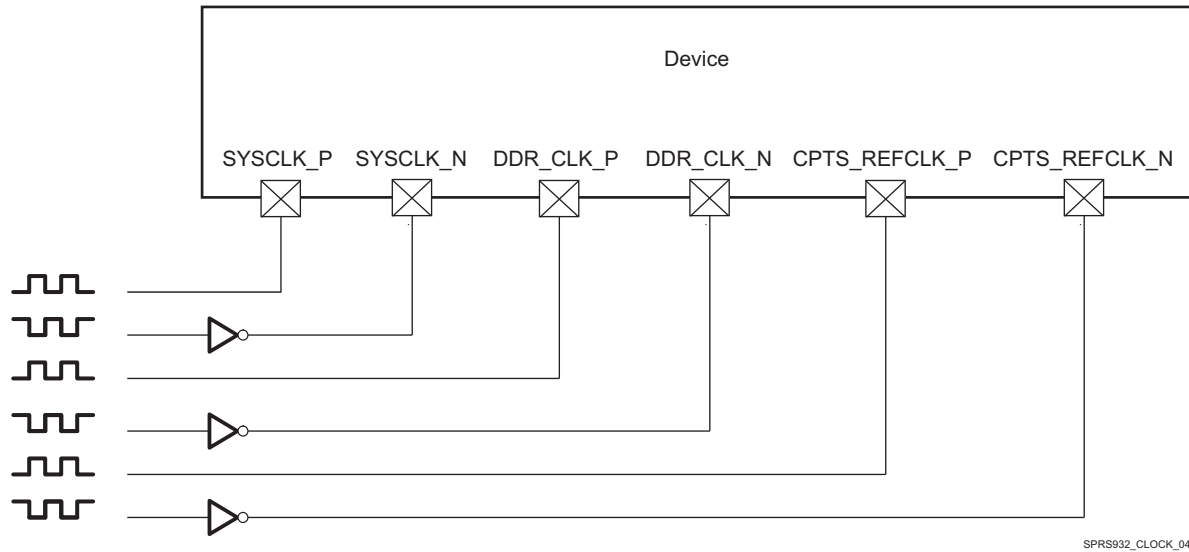
Figure 5-14. LVDS-Compatible Clock Input
