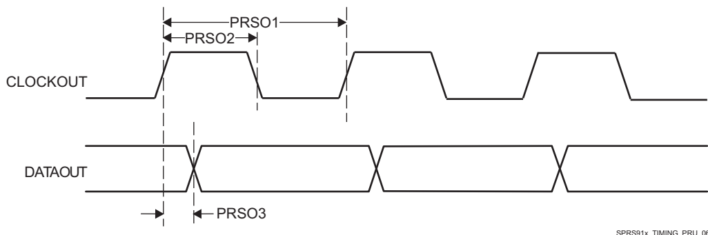
Figure 5-67. PRU-ICSS PRU Shift Out Timing
