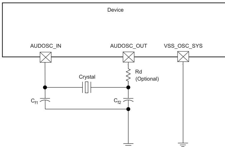
Figure 5-17. Crystal Implementation (1)
