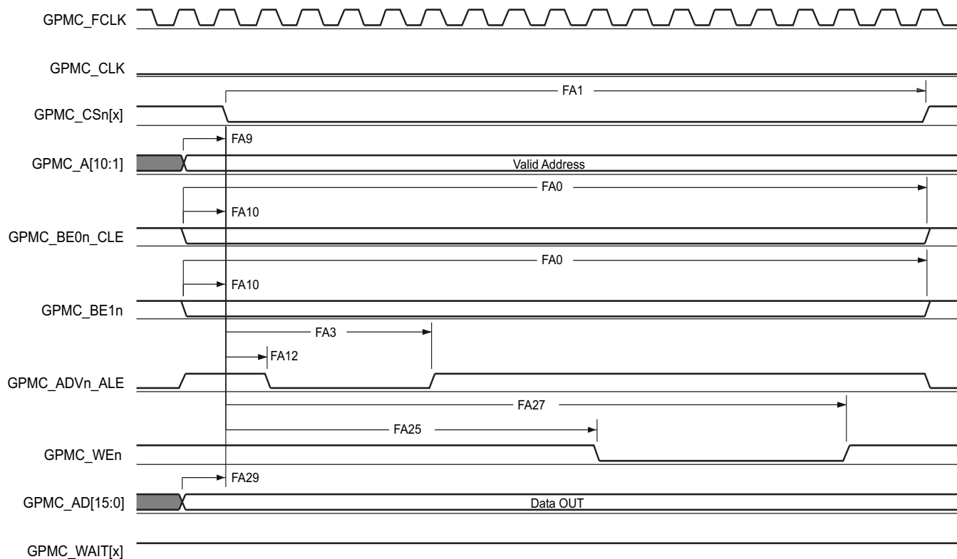
Figure 5-44. GPMC and NOR Flash—Asynchronous Write—Single Word
