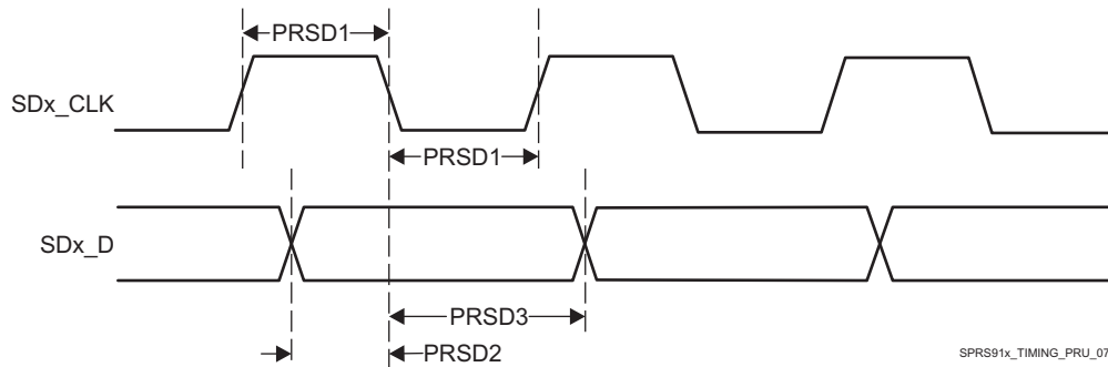
Figure 5-79. PRU-ICSS PRU SD_CLK Falling Active Edge
