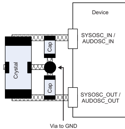
Figure 7-25. SYSOSC and AUDIOOSC PCB requirements
