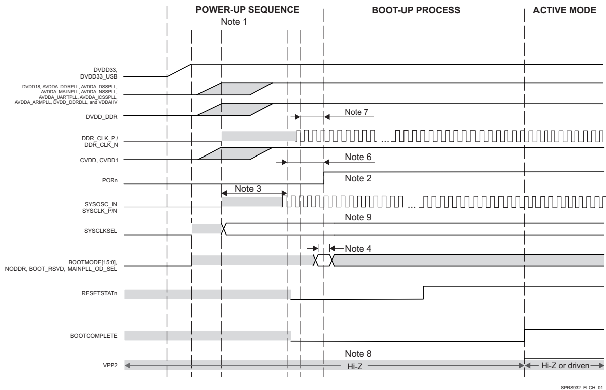
Figure 5-3. Power-Up Sequencing
