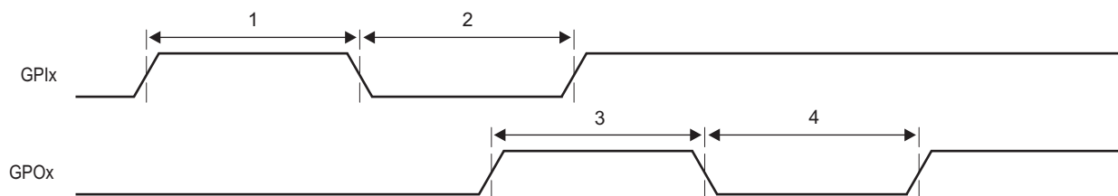
Figure 9-50 GPIO Timing
