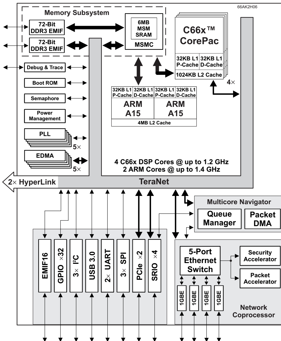
Figure 1-2 Functional Block Diagram for 66AK2H06
