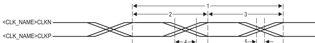
Figure 9-22 Main PLL Transition Time
