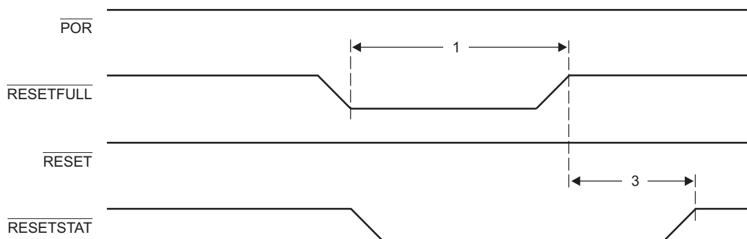
Figure 9-4 \overline{\text{RESETFULL}} Reset Timing
