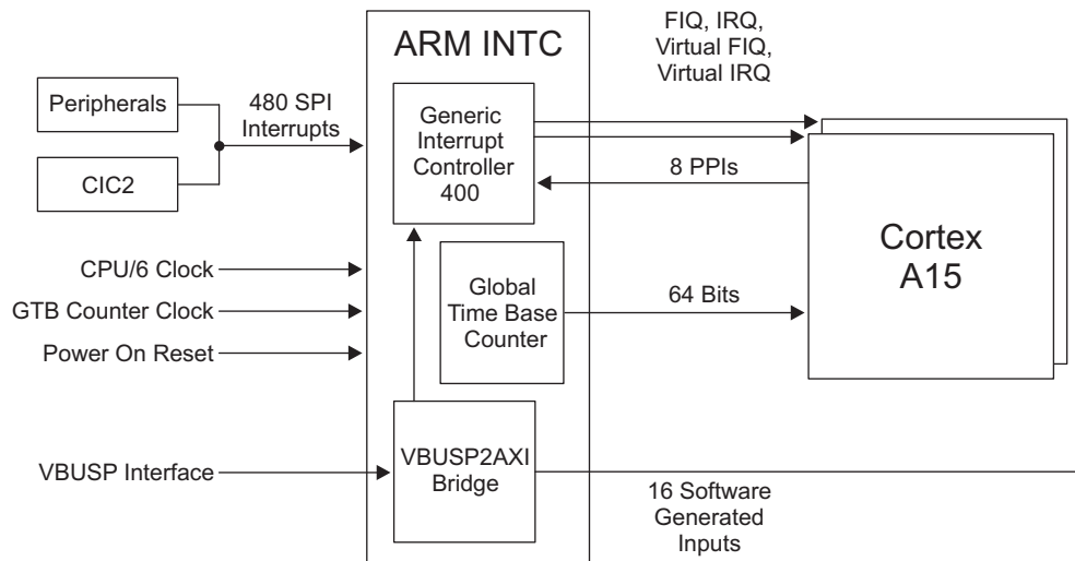
Figure 3-2 ARM Interrupt Controller for 2 Cortex-A15 Processor Cores
