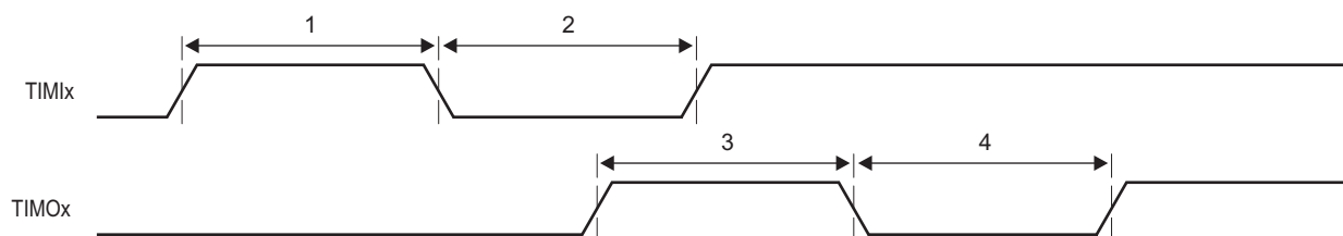
Figure 9-49 Timer Timing
