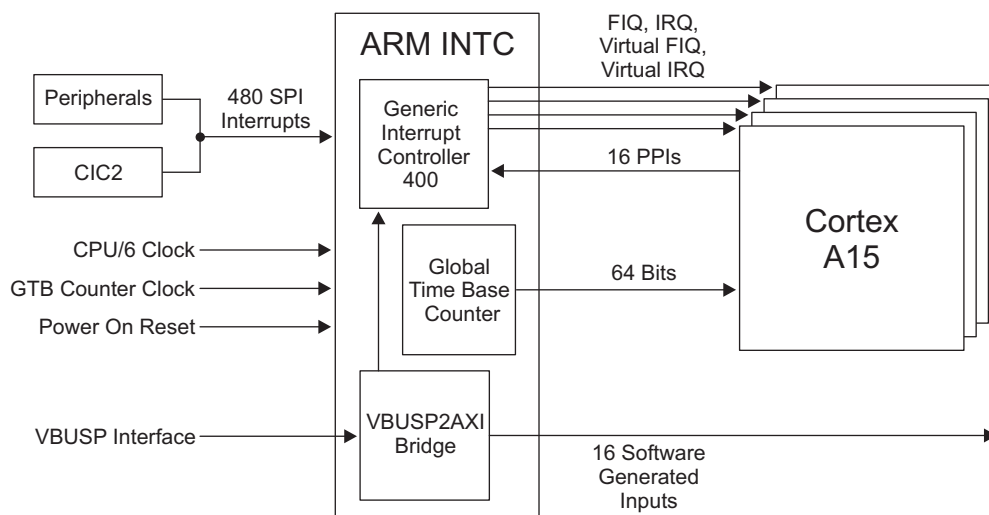
Figure 3-3 ARM Interrupt Controller for 4 Cortex-A15 Processor Cores
