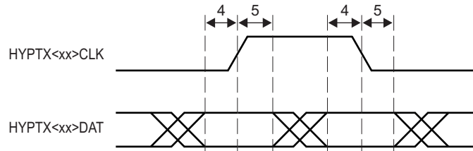
Figure 9-38 HyperLink Station Management Transmit Timing
