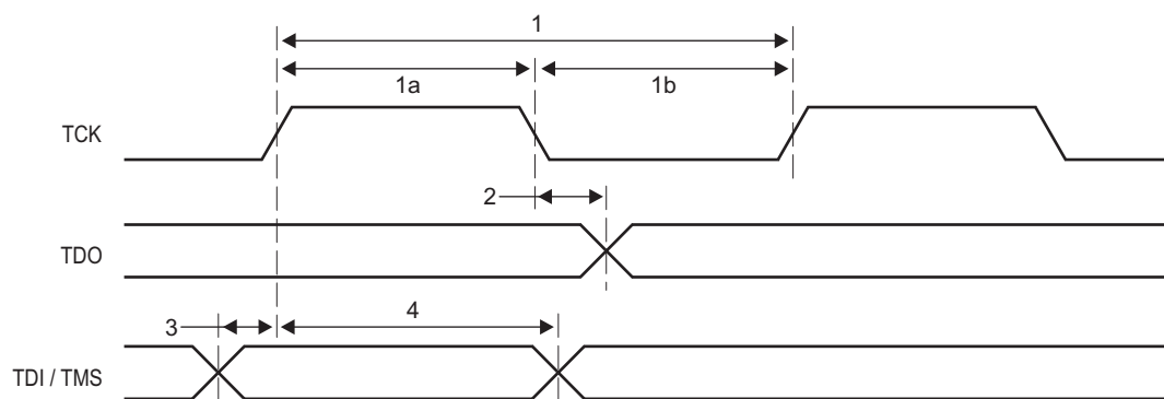
Figure 9-56 JTAG Test-Port Timing
