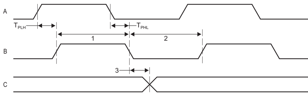
Figure 9-55 Trace Timing
