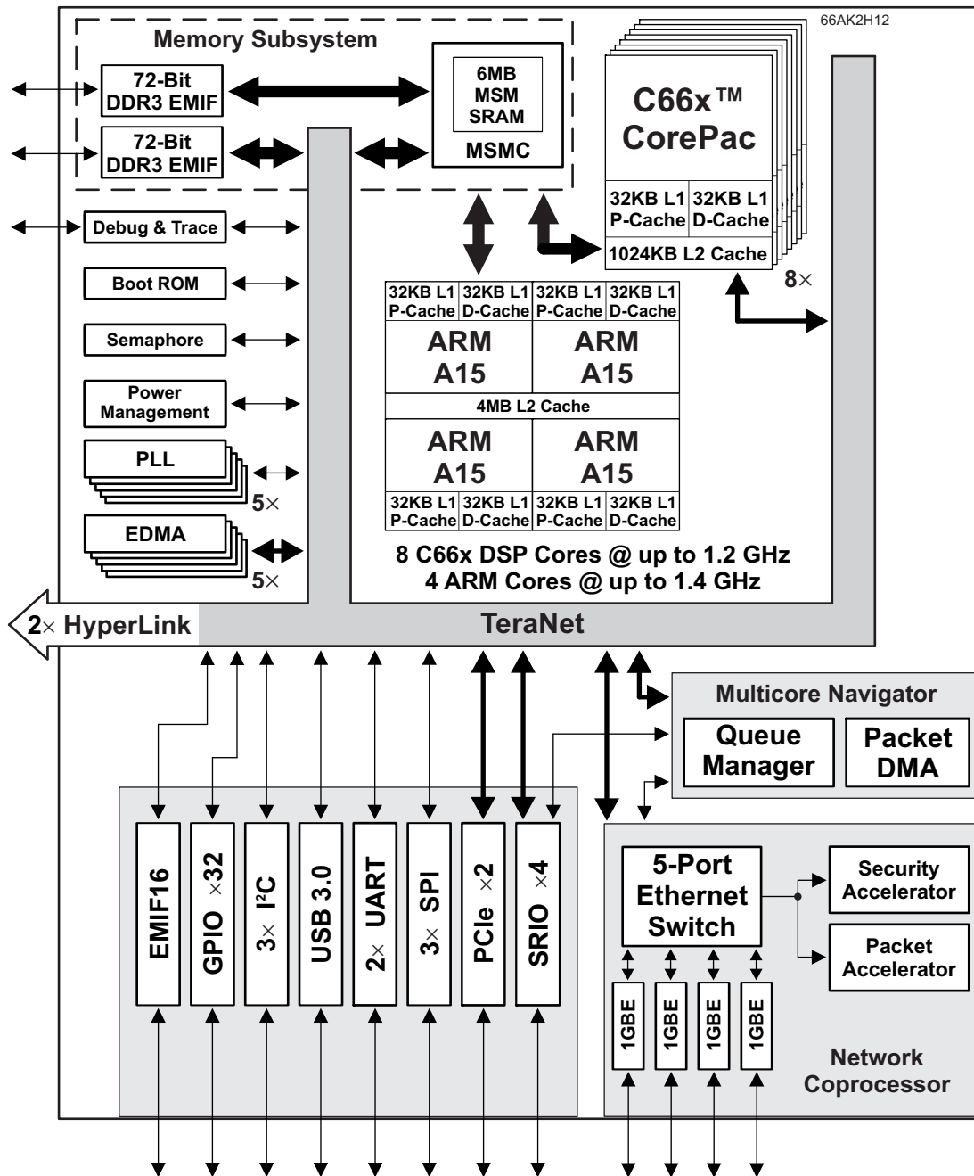
Figure 1-1 Functional Block Diagram for 66AK2H12
