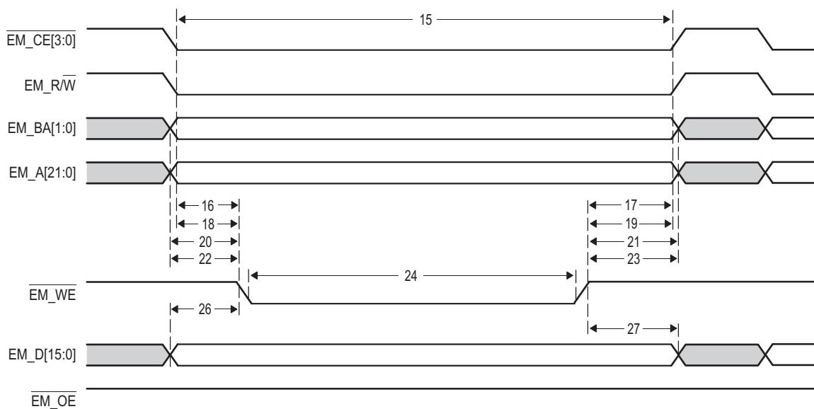
Figure 9-52 EMIF16 Asynchronous Memory Write Timing Diagram
