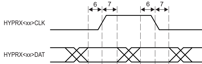
Figure 9-39 HyperLink Station Management Receive Timing
