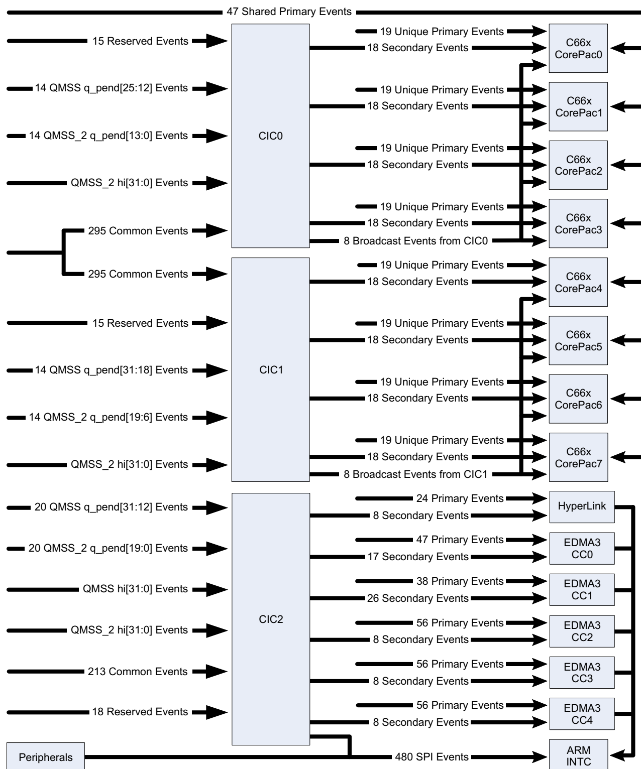
Figure 5-4 Interrupt Topology
