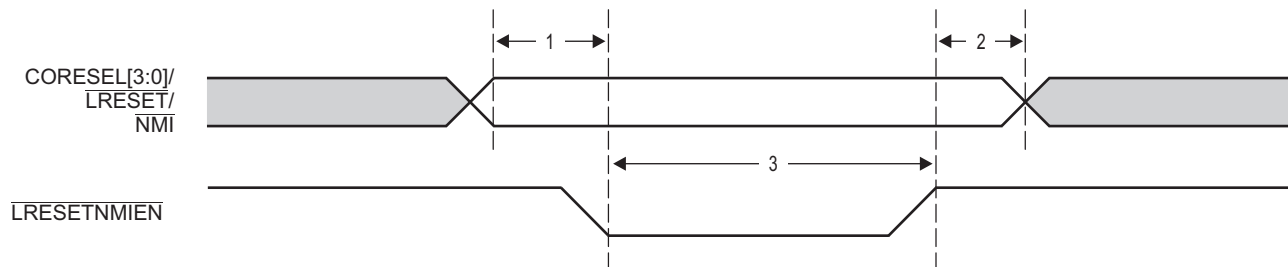
Figure 9-31 \overline{\text{NMI}} and \overline{\text{LRESET}} Timing
