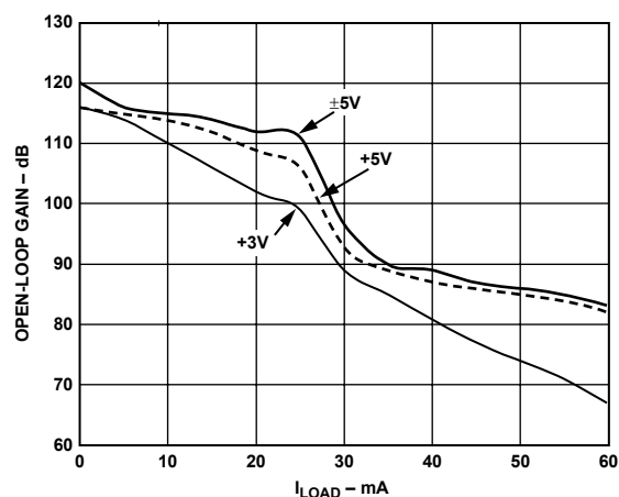
Figure 44. Open-Loop Gain vs. Load Current
