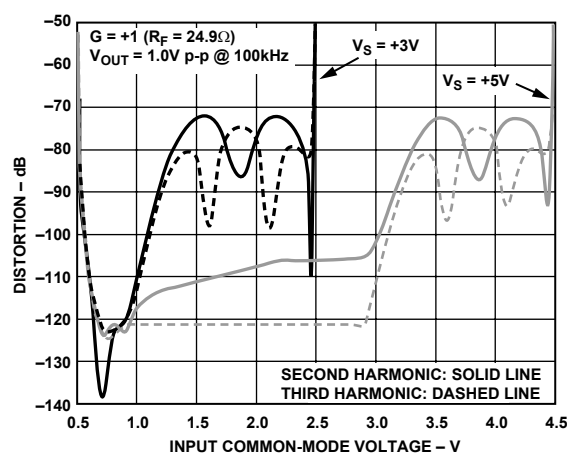
Figure 21. Harmonic Distortion vs. Input Common-Mode Voltage, SELECT = Tri\text{-}State\text{ or }Open
