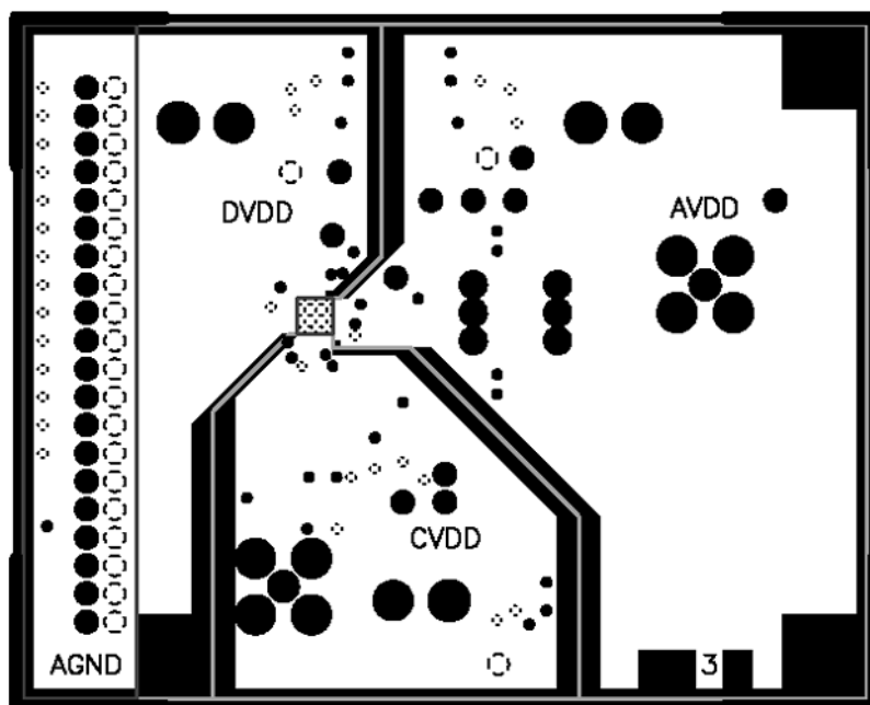
Figure 33. LFCSP Evaluation Board Layout—Power Plane
