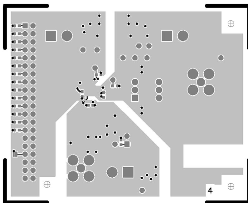
Figure 31. LFCSP Evaluation Board Layout—Secondary Side
