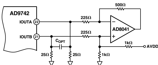
Figure 14. Single-Supply DC Differential Coupled Circuit
