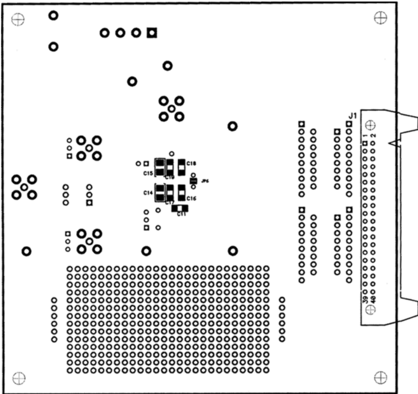
Figure 26. SOIC Evaluation Board Assembly—Secondary Side
