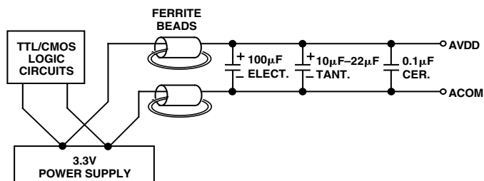
Figure 18. Differential LC Filter for Single 3.3 V Applications
