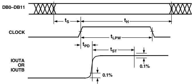
Figure 1. Timing Diagram
