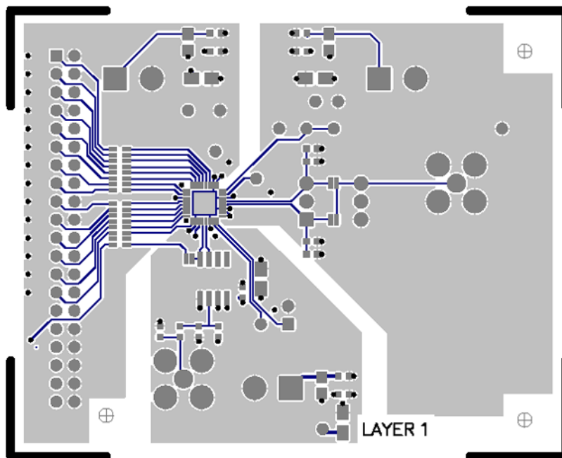
Figure 30. LFCSP Evaluation Board Layout—Primary Side
