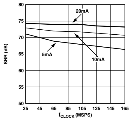
TPC 8. SNR vs. f_{CLOCK} and I_{OUTFS} @ f_{OUT} = 5 MHz and 0 dBFS
