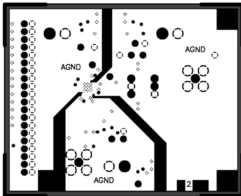
Figure 32. LFCSP Evaluation Board Layout—Ground Plane
