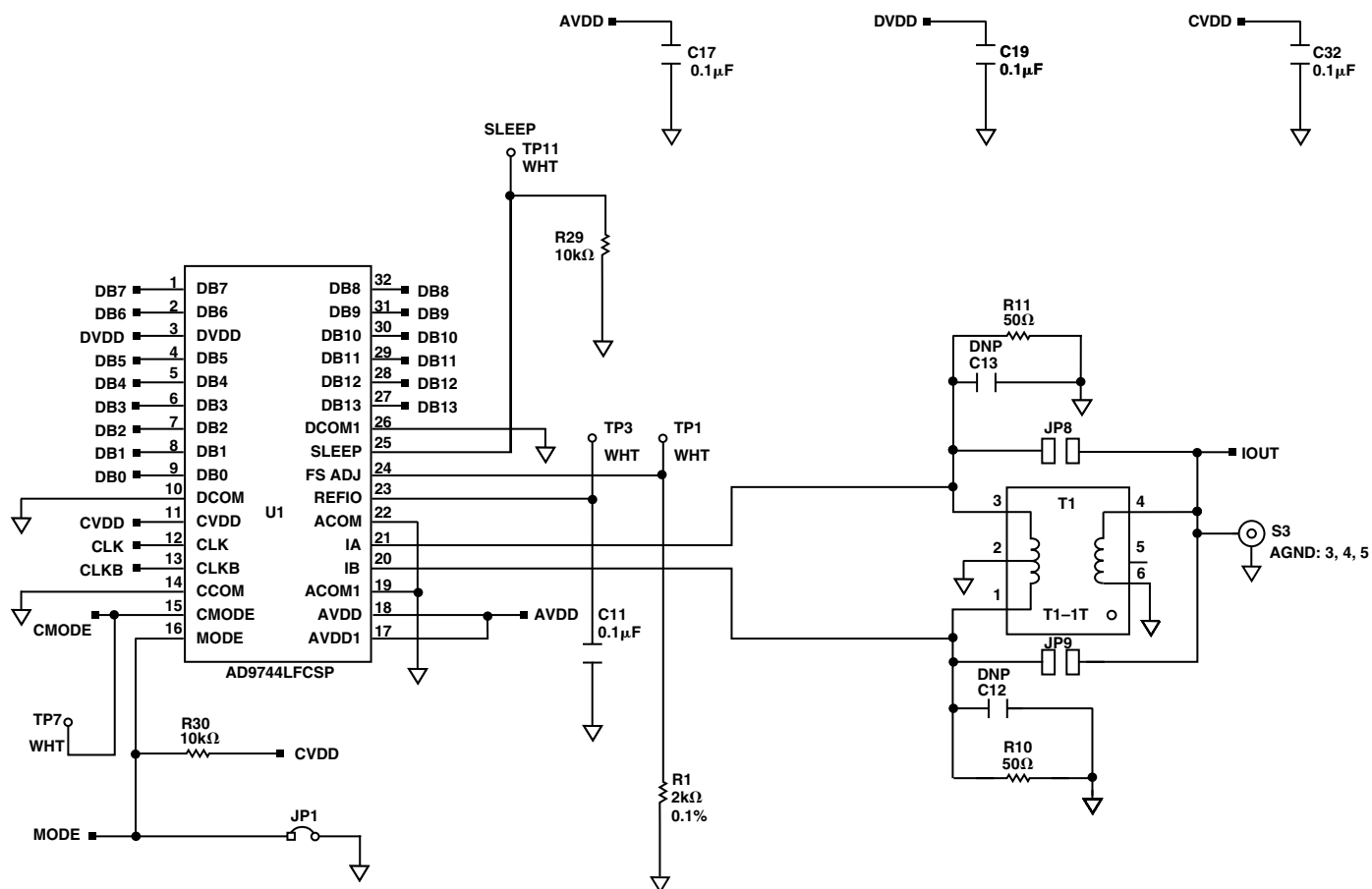
Figure 28. LFCSP Evaluation Board Schematic—Output Signal Conditioning
