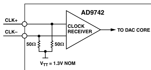
Figure 7. Clock Termination in PECL Mode
