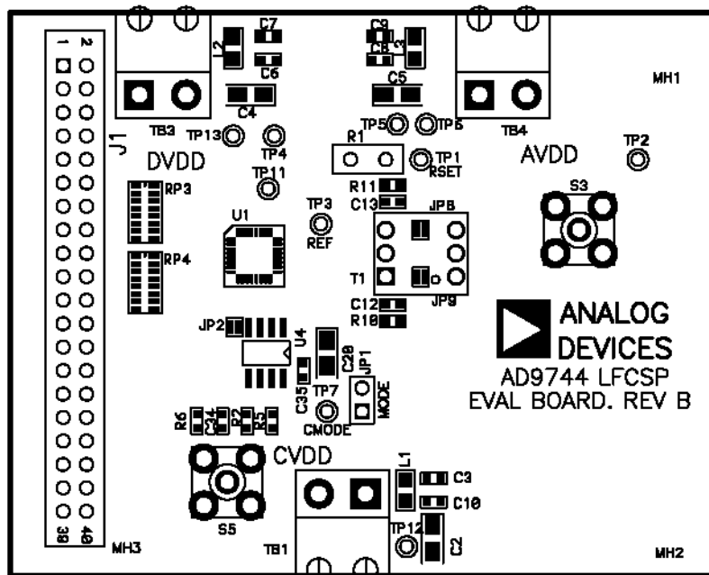
Figure 34. LFCSP Evaluation Board Layout Assembly—Primary Side
