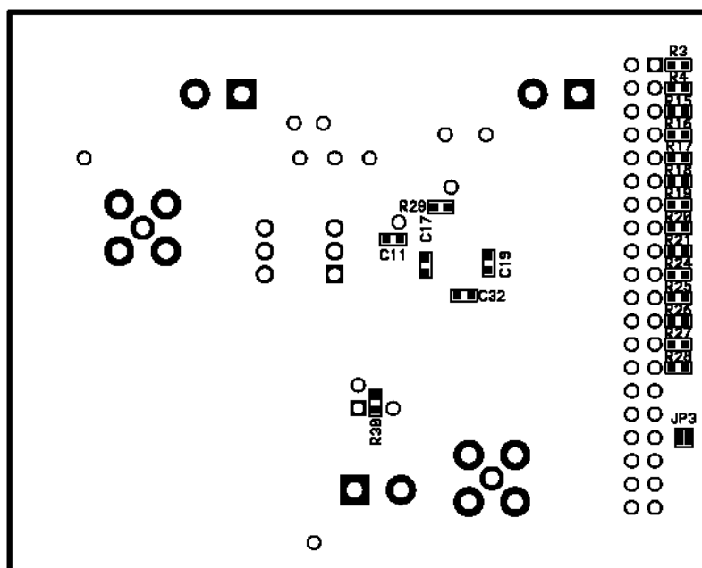
Figure 35. LFCSP Evaluation Board Layout Assembly—Secondary Side
