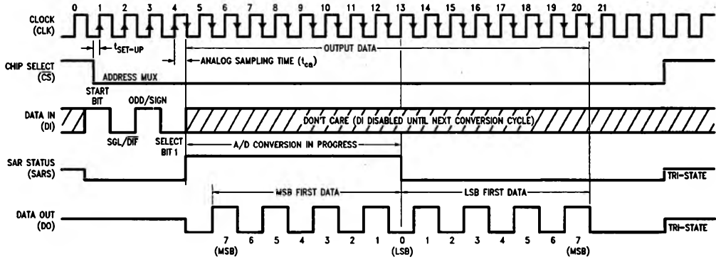
ADC08134 Timing
