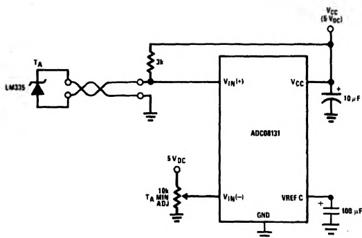
Low-Cost Remote Temperature Sensor
