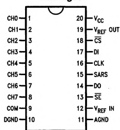
ADC08138 Dual-In-Line and Small Outline Packages
