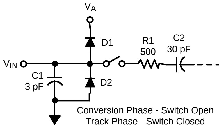
Figure 52. Equivalent Input Circuit
