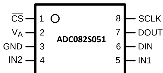
Figure 1. VSSOP Package See Package Number DGK0008A
