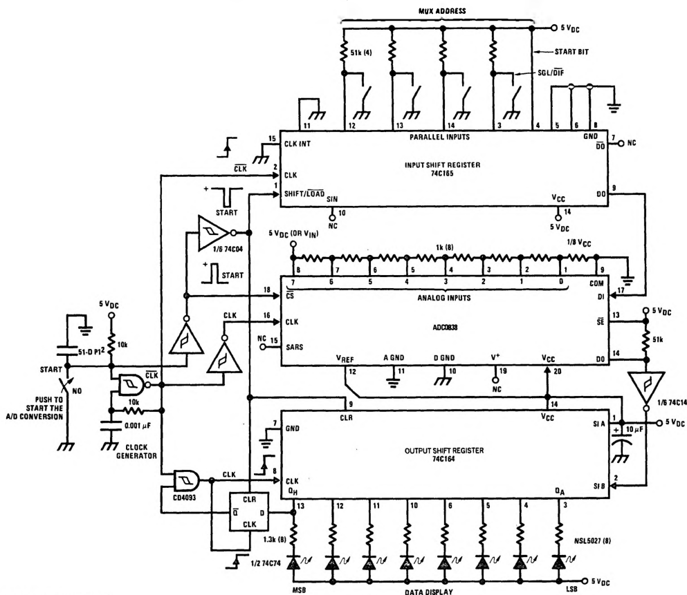
A “Stand-Alone” Hook-Up for ADC0838 Evaluation
