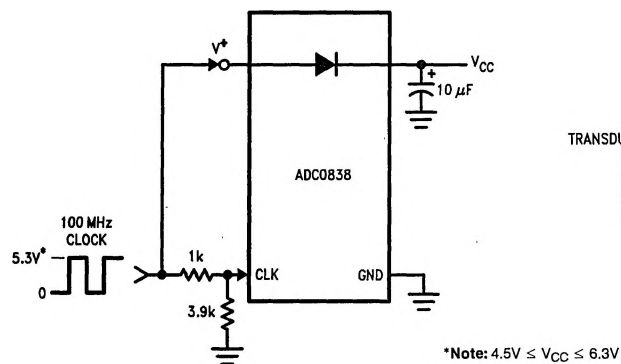
FIGURE 6. Generating V_{CC} from the Converter Clock
