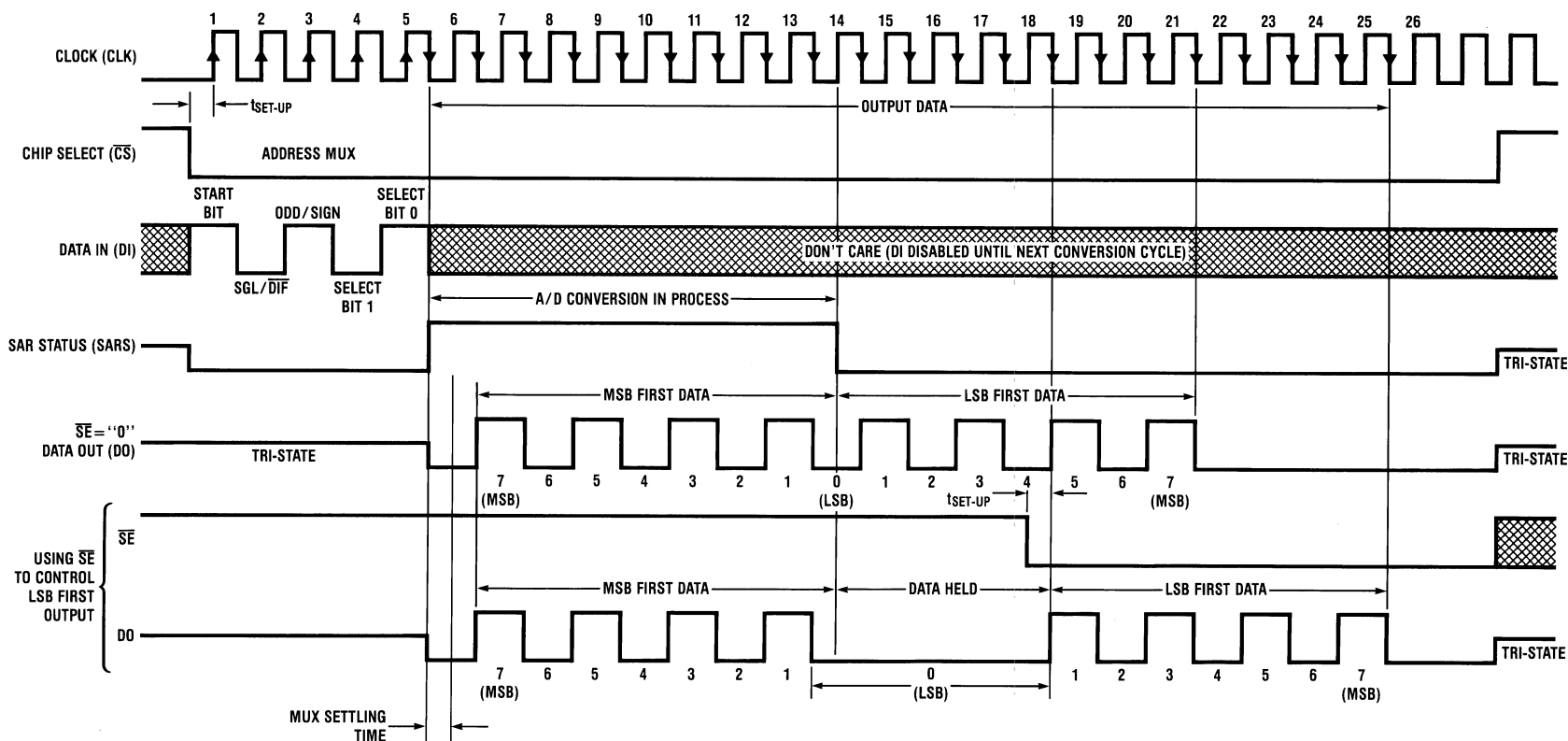
Figure 21. ADC0838-N Timing
