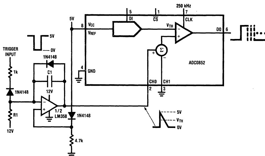
FIGURE 17. Pulse-Width Modulator
