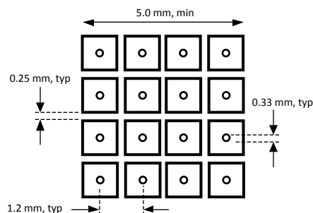
Figure 51. Recommended Package Exposed Pad Land Pattern
