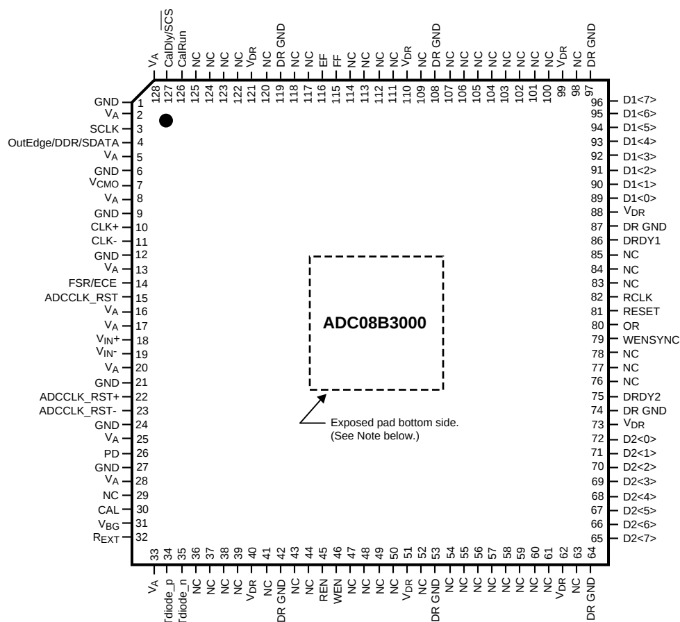
Figure 1. HLQFP Package See Package Number NNB0128A
