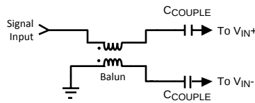
Figure 45. Single-Ended to Differential Signal Conversion with a Balun
