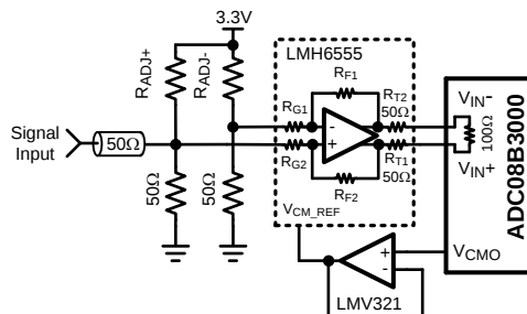
Figure 46. Example of Servoing the Analog Input with V_{CMO}
