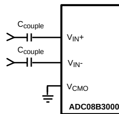
Figure 44. Differential Data Input Connection
