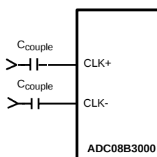
Figure 47. Differential Sample Clock Connection
