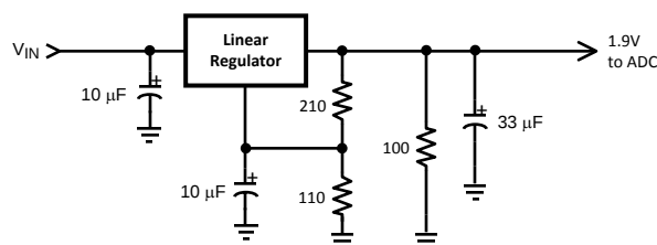
Figure 50. Non-Spiking Power Supply
