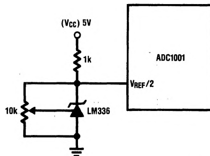
FIGURE 3. Full-Scale Adjust
