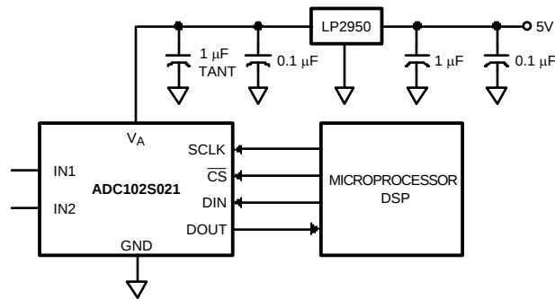
Figure 8. Typical Application Circuit
