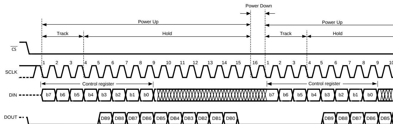
Figure 1. ADC102S021 Operational Timing Diagram
