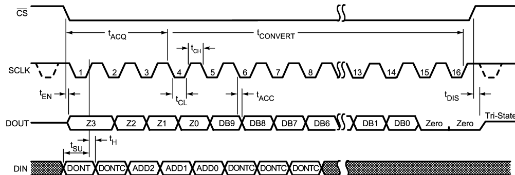
Figure 3. ADC102S021 Serial Timing Diagram
