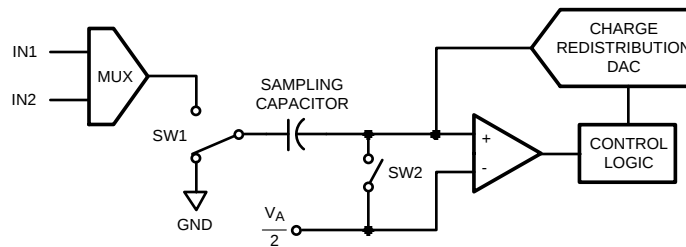
Figure 6. ADC102S021 in Hold Mode
