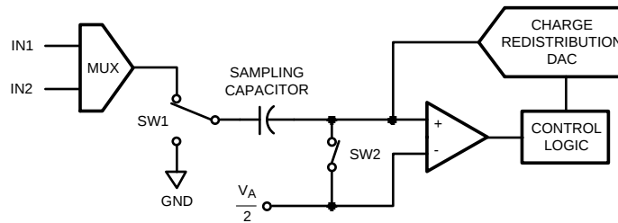
Figure 5. ADC102S021 in Track Mode
