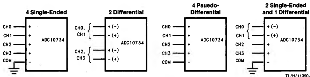
FIGURE 12. Analog Input Multiplexer Options
