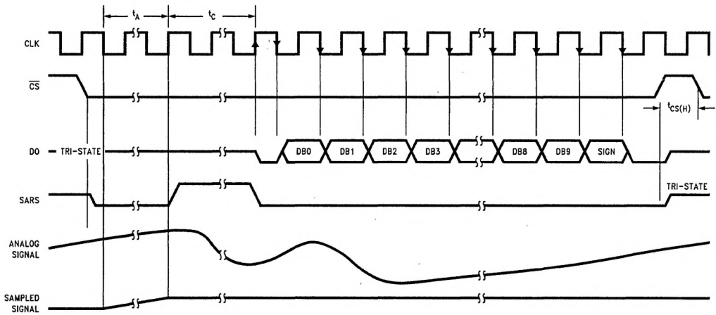
FIGURE 7. ADC10731 \overline{CS} Low during Conversion
