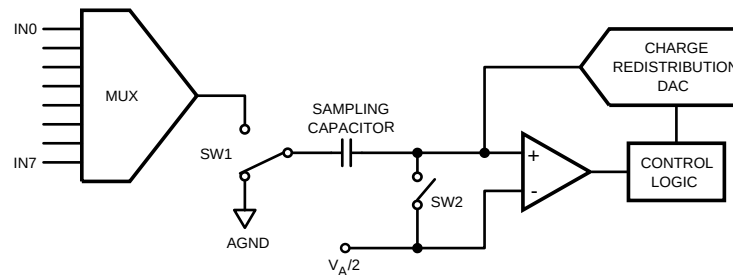
Figure 5. ADC108S102 in Hold Mode
