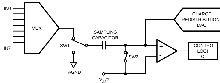
Figure 4. ADC108S102 in Track Mode
