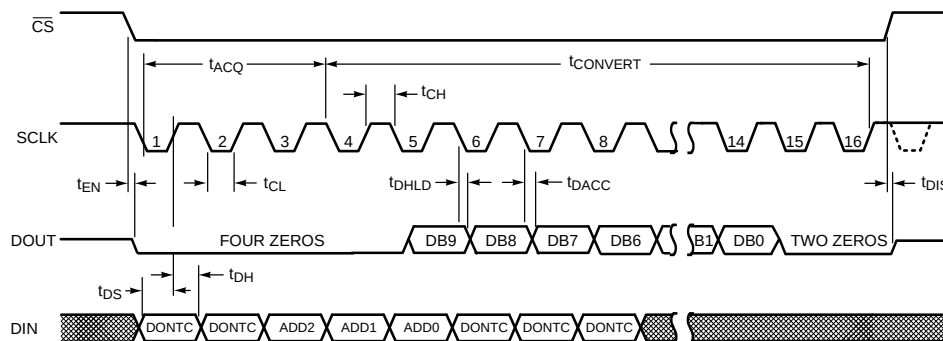
Figure 2. ADC108S102 Serial Timing Diagram
