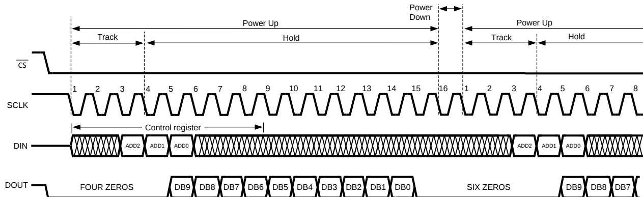
Figure 1. ADC108S102 Operational Timing Diagram
