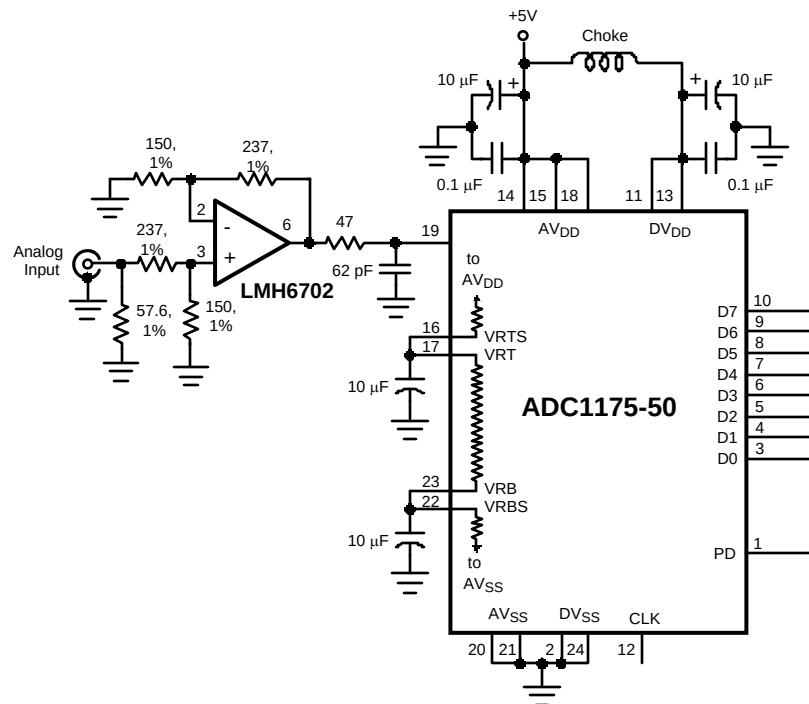
Figure 5. Driving the ADC1175-50
