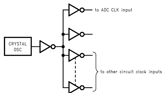
Figure 8. Isolating the ADC Clock from Digital Circuitry
