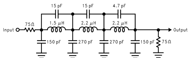
Figure 10. An 11 MHz Low Pass filter to eliminate harmonics at the signal input
