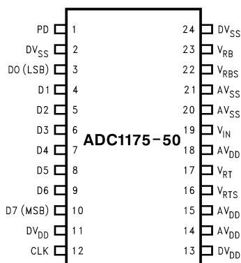
Figure 1. 24-pin SOIC and TSSOP - Top View SOIC obsolete. Shown for reference only
