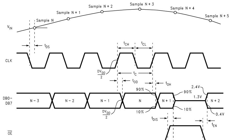
Figure 3. ADC1175-50 Timing Diagram
