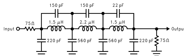
Figure 9. A 5.5 MHz Low Pass filter to eliminate harmonics at the signal input
