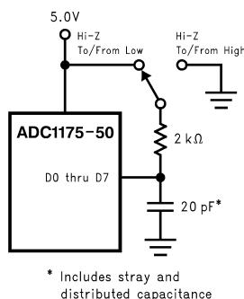
Figure 4. t_{EN} , t_{DIS} Test Circuit
