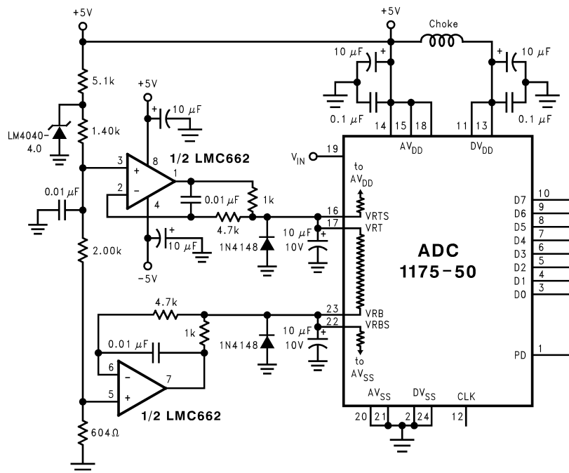
Figure 6. Better Defining the ADC Reference Voltage.
