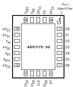
Figure 2. 24-pin LLP (CSP) - Bottom View
