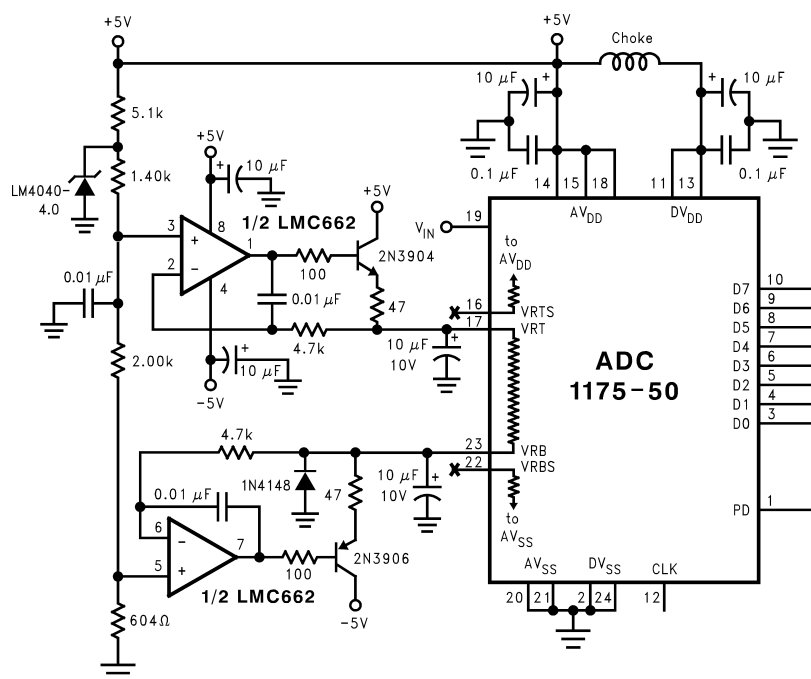
Figure 6. Better Defining the ADC Reference Voltage.
