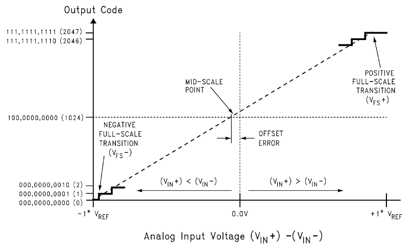
Figure 2. Transfer Characteristic (Offset Binary Format)
