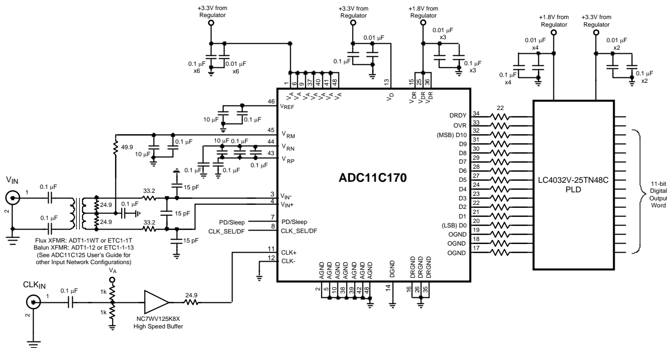
If 14-bit compatibility is not required do not connect pins 17 - 19. If 12-bit compatibility if not required do not connect pin 19.
