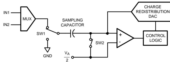
Figure 5. ADC122S021 in Track Mode
