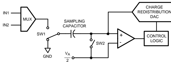
Figure 6. ADC122S021 in Hold Mode
