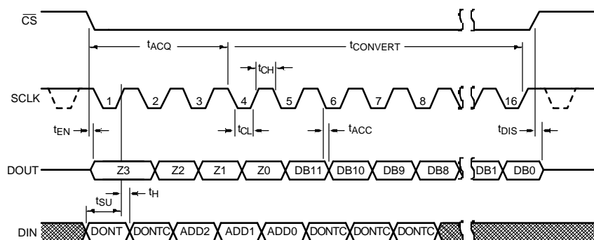
Figure 3. ADC122S021 Serial Timing Diagram
