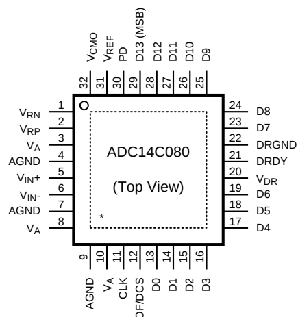
Figure 1. WQFN Package See Package Number RTV0032A
