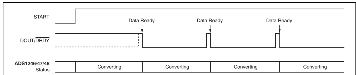
Figure 68. Timing for Conversion with START Pin High
