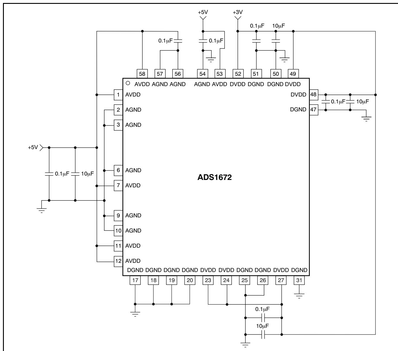
Figure 38. Power-Supply Decoupling
