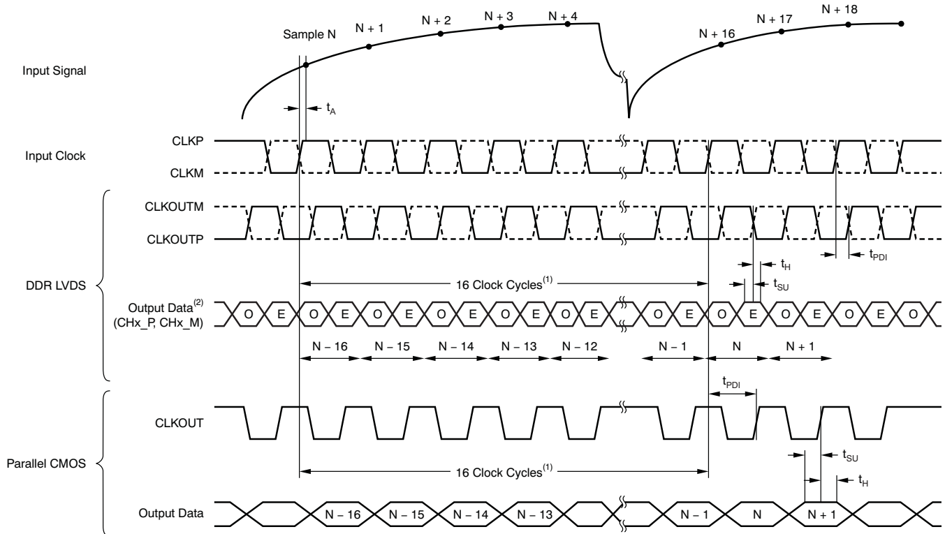
Figure 5. Latency Diagram
