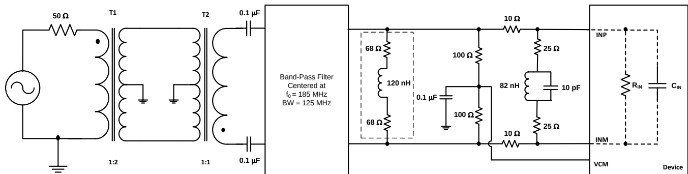
Figure 48. Driving Circuit for a 100- \Omega Source Impedance and Input Frequencies in the Second Nyquist Zone
