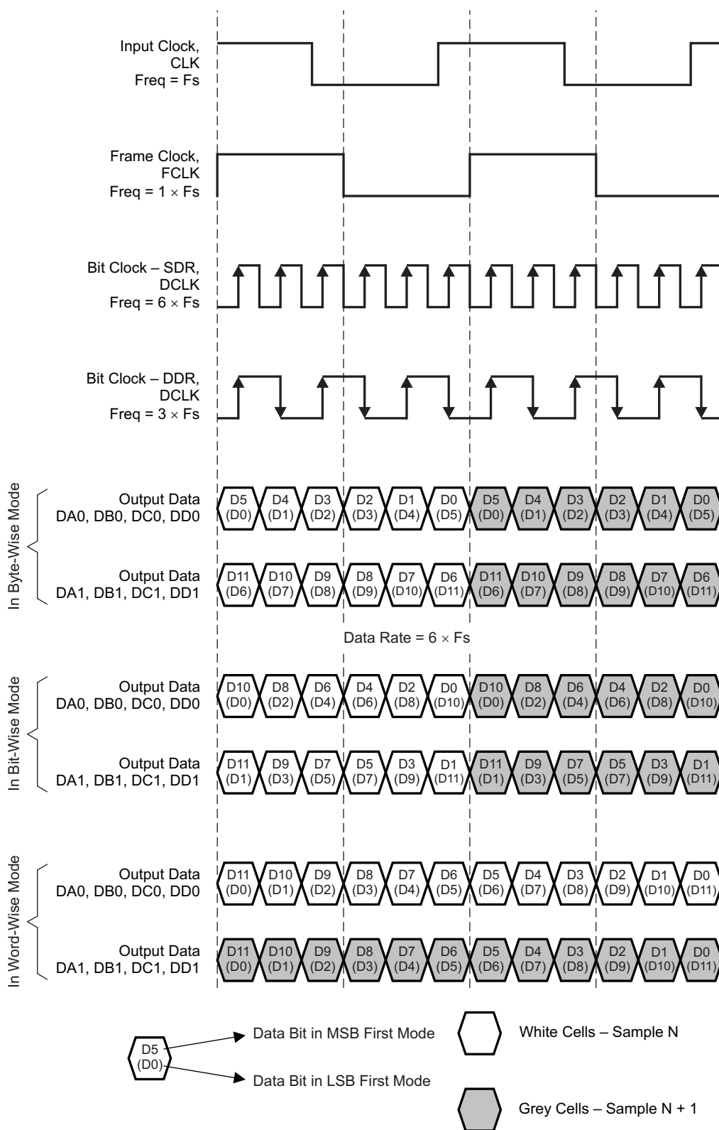
Figure 76. 2-Wire Interface 12x Serialization
