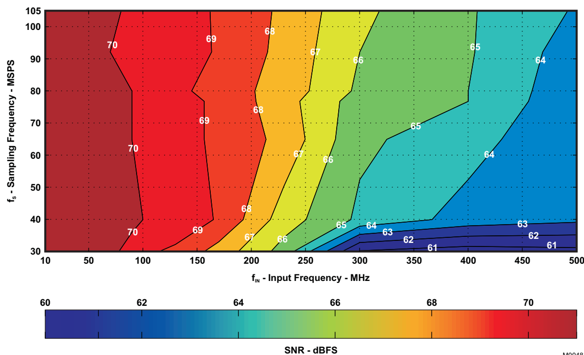
Figure 63. SNR Contour (3.5 dB coarse gain)
