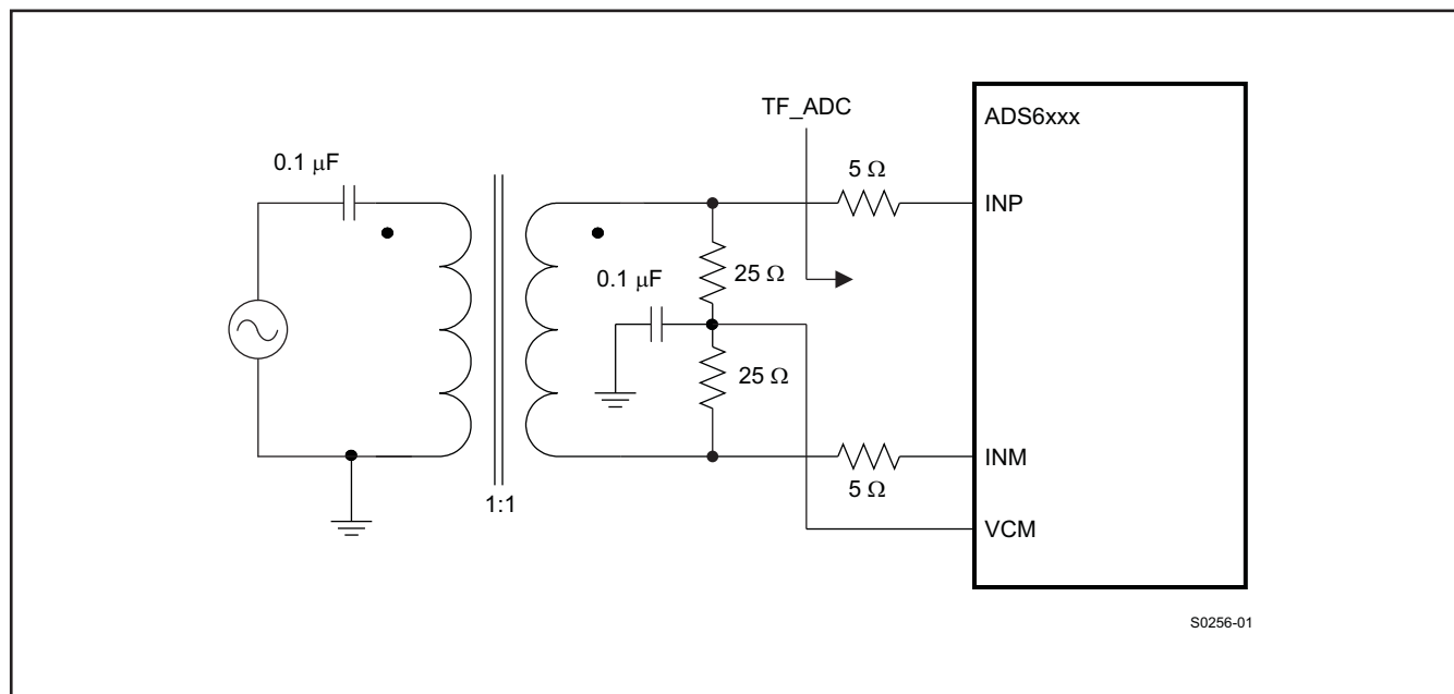
Figure 67. Single Transformer Drive Circuit
