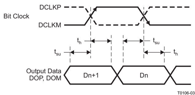
Figure 2. LVDS Timings
