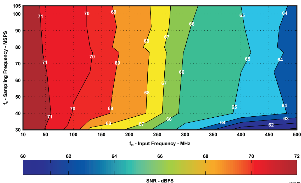
Figure 62. SNR Contour (no gain)
