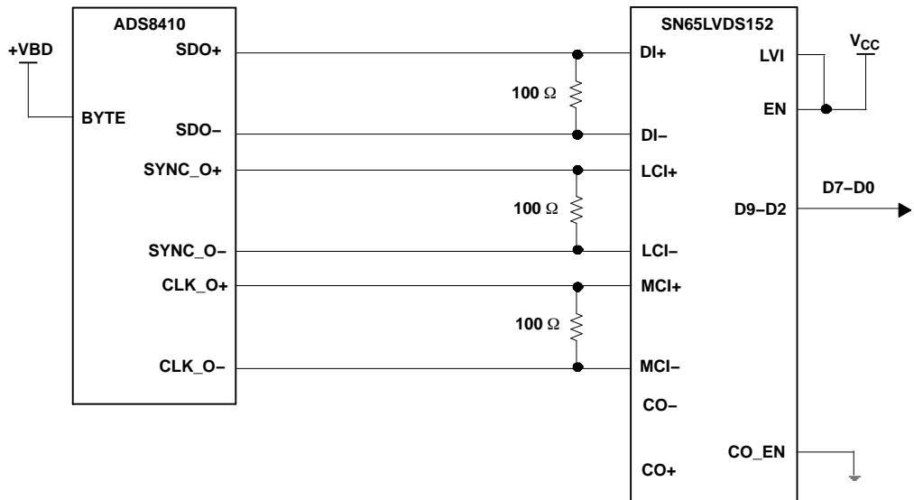
Figure 21. 8-Bit Data De-Serialization While BYTE = 1, Data
