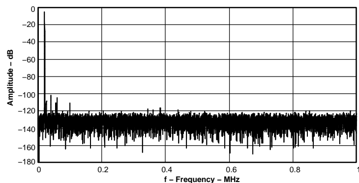
Figure 51. Typical FFT
