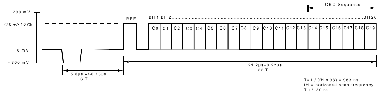
Fig xx. CGMS Waveform
