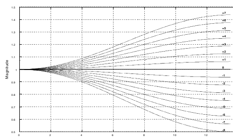
Figure xx Frequency response in Sharpness Filter mode with K_a=+3 and K_b=+7 when step input is applied
