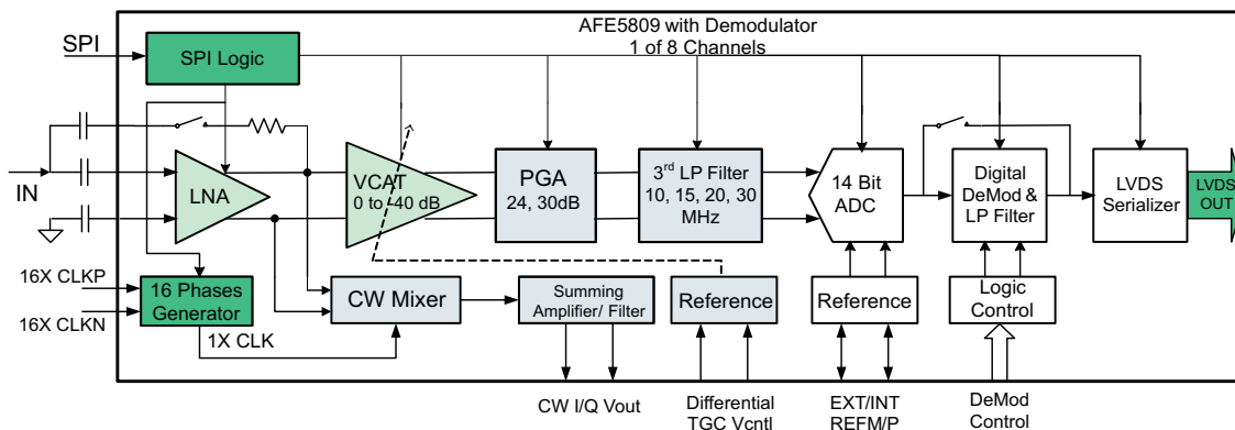
Figure 1. Block Diagram
