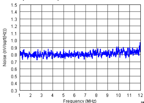
Figure 28. IRN, PGA = 24 dB and Low Noise Mode
