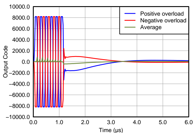
Figure 56. Pulse Inversion, V_N = 2 Vpp, PRF = 1 KHz, Gain = 21 dB
