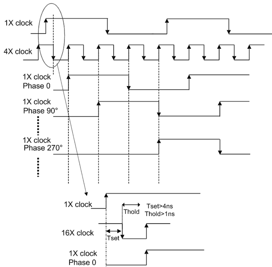
Figure 82. 8 × f cw and 4 × f cw Timing Diagram
