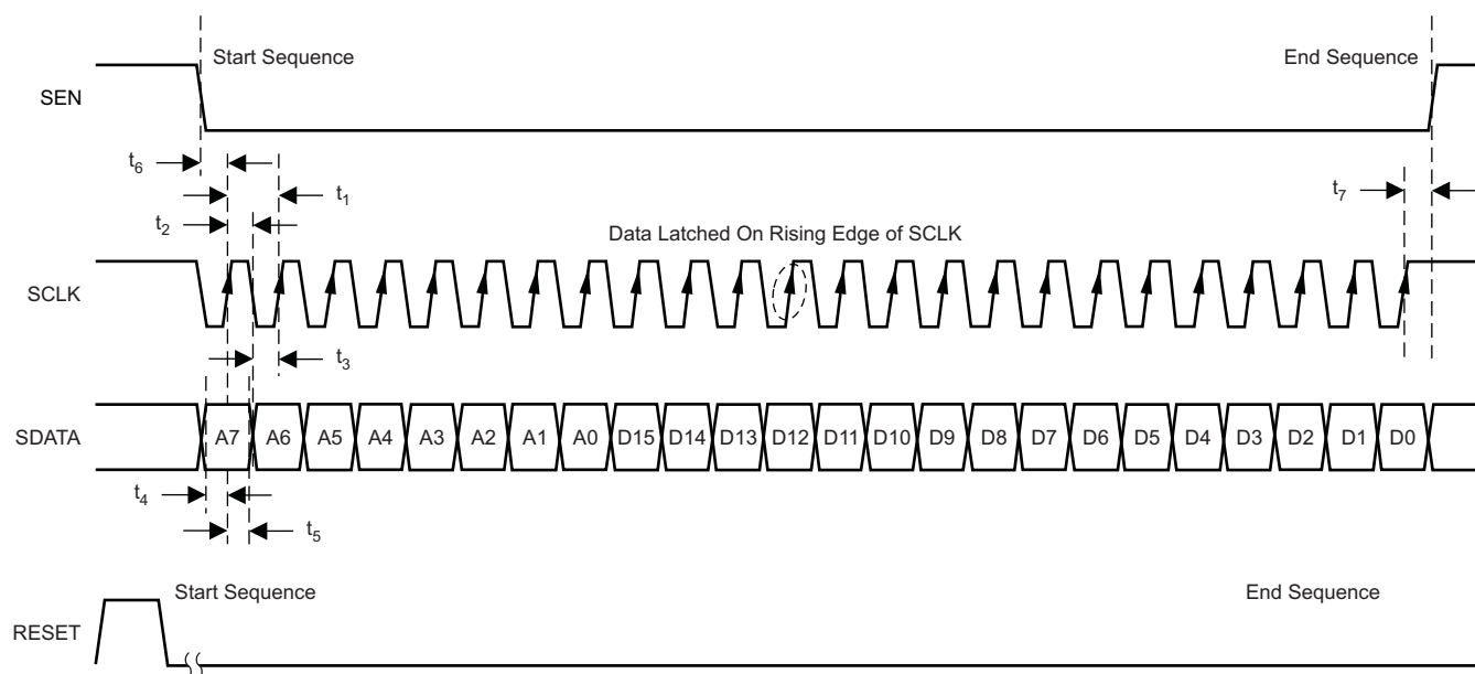
Figure 62. SPI Timing
