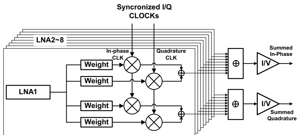
Figure 83. Block Diagram of 1 × f cw mode
