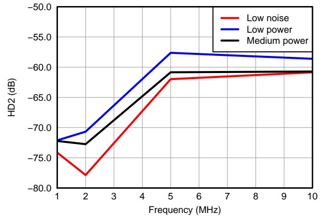
Figure 38. HD2 vs Frequency, V_{IN} = 500 \text{ mVpp} and V_{OUT} = -1 \text{ dBFS}
