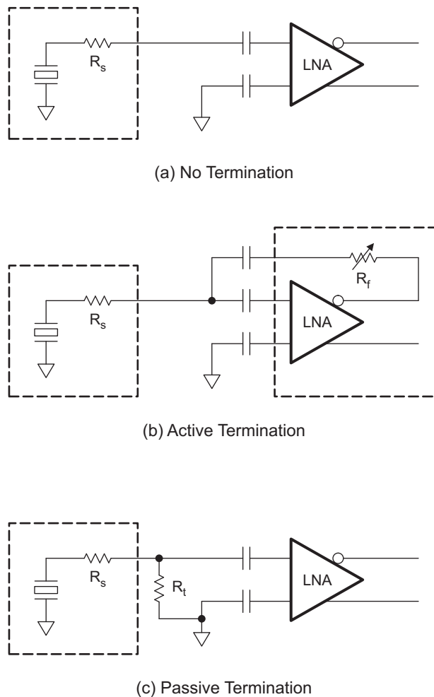
Figure 94. Termination Configurations
