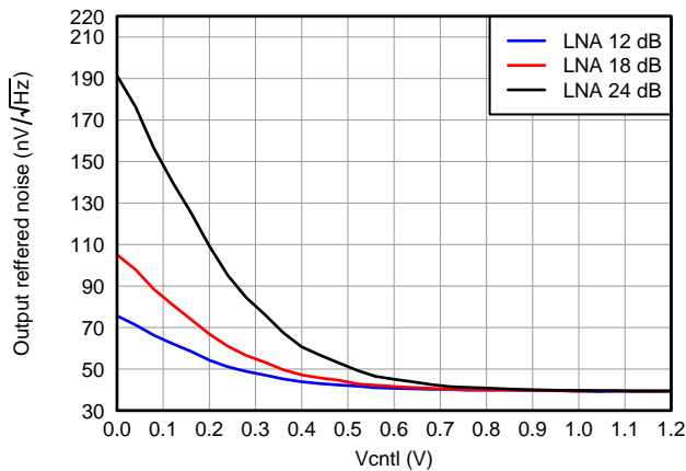
Figure 25. ORN, PGA = 24 dB and Low Noise Mode
