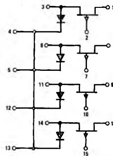
UNCOMMITTED DRAINS TL/H/5859-1
