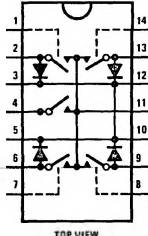
AH5010C MUX Switches (4-Channel Version Shown) Order Number AH5010CN
