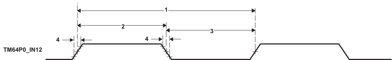
Figure 5-42. Timer Timing
