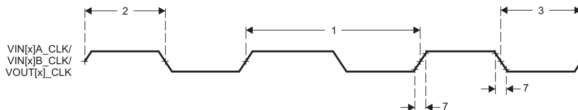
Figure 8-68. HDVPSS Clock Timing
