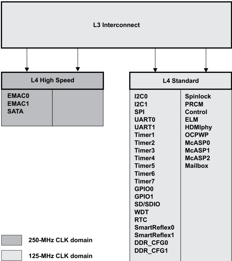
Figure 5-2. L4 Architecture
