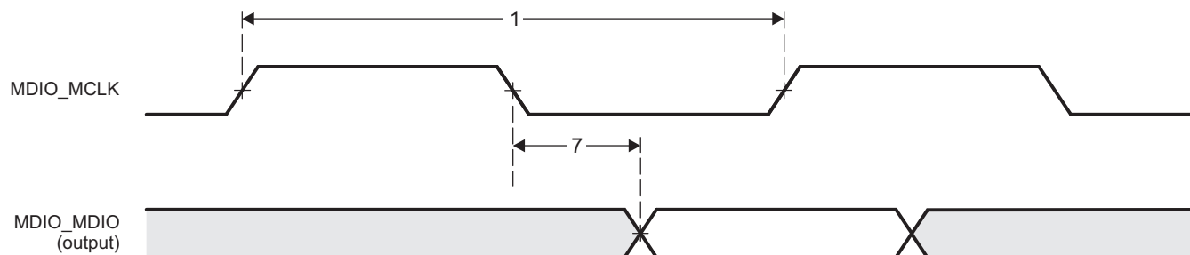
Figure 8-48. MDIO Output Timing
