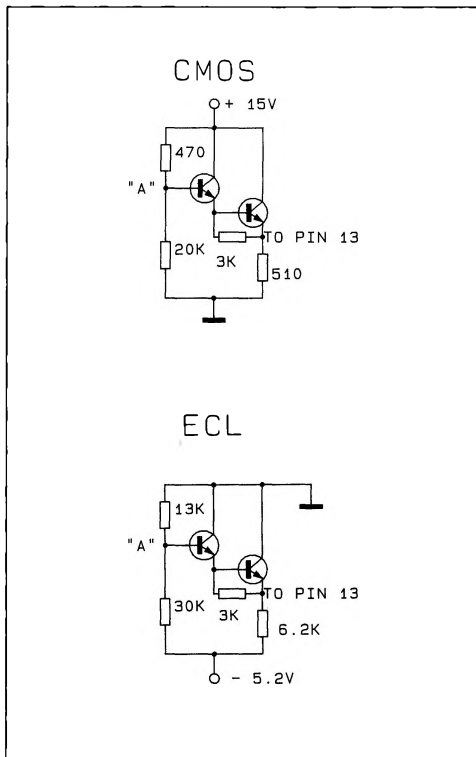
Fig. 6 - Interfacing Circuits
