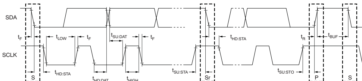
Figure 1. Timing Specification
