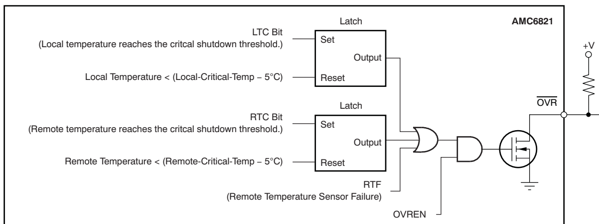
Figure 30. \overline{\text{OVR}} Pin
