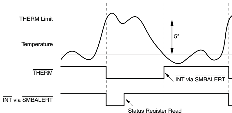
Figure 23. Operation of the THERM Interrupt and the THERM Pin
