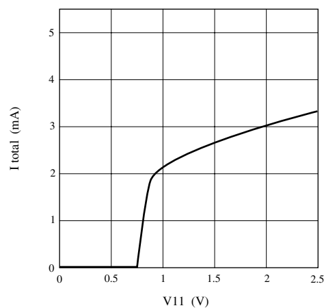
12. V_{CC} - I_{total}
