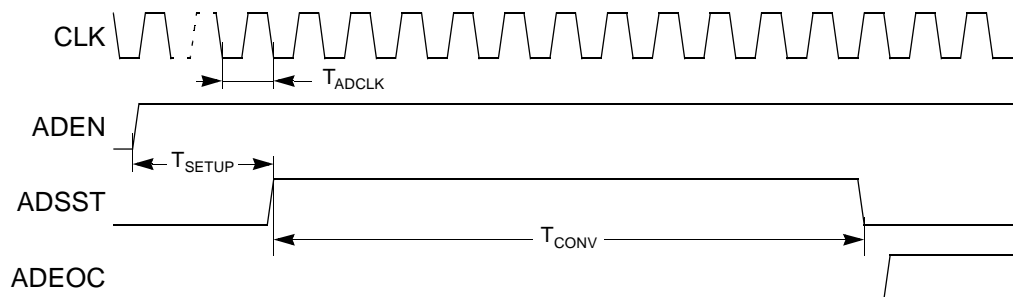
Figure 130. Timing Diagram
