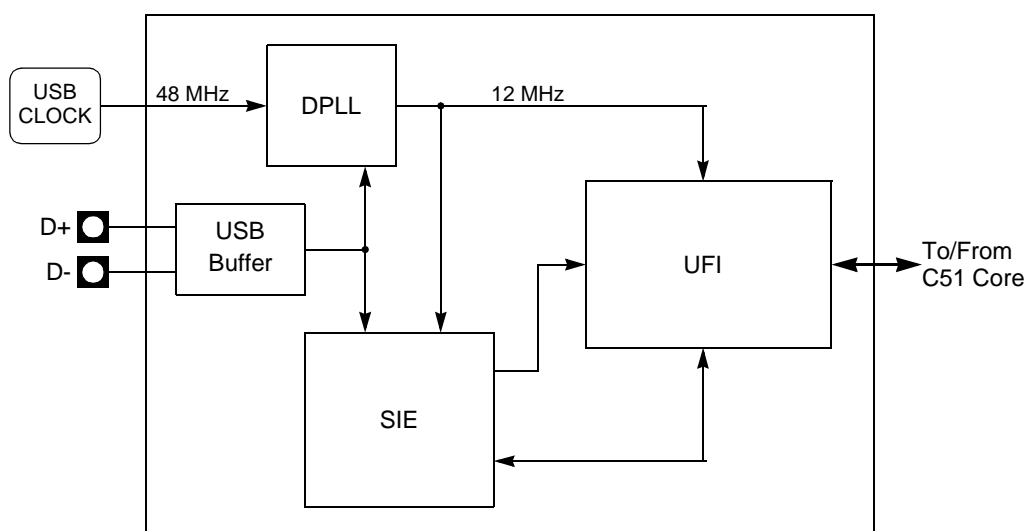
Figure 55. USB Device Controller Block Diagram
