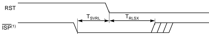
Figure 155. FLASH Memory - ISP Waveforms
