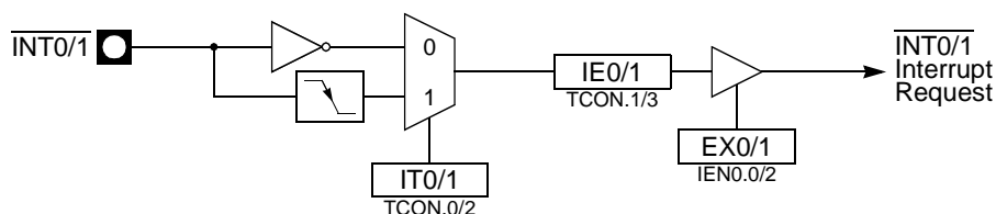
Figure 22. \overline{\text{INT1:0}} Input Circuitry
