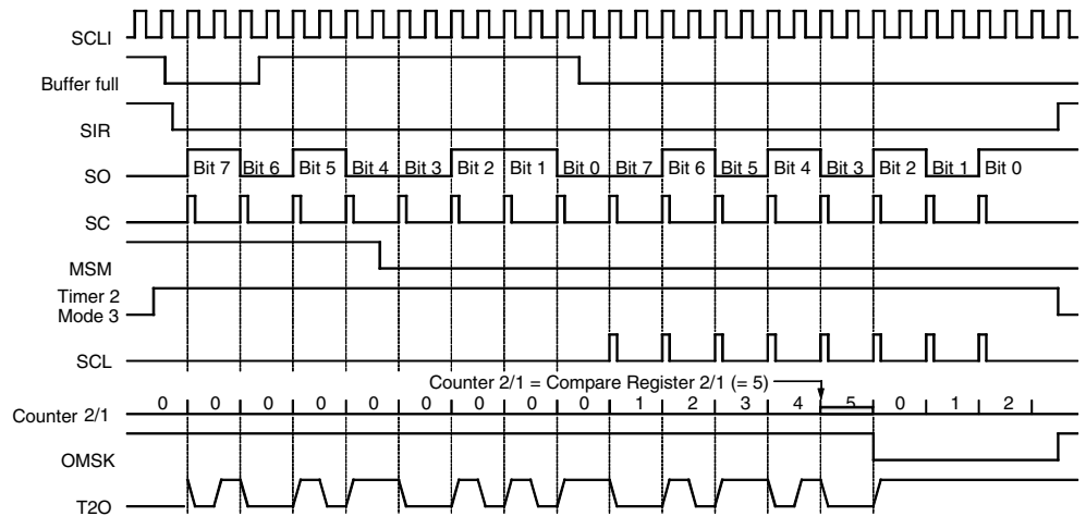
Figure 73. Bi-phase Modulation 2
