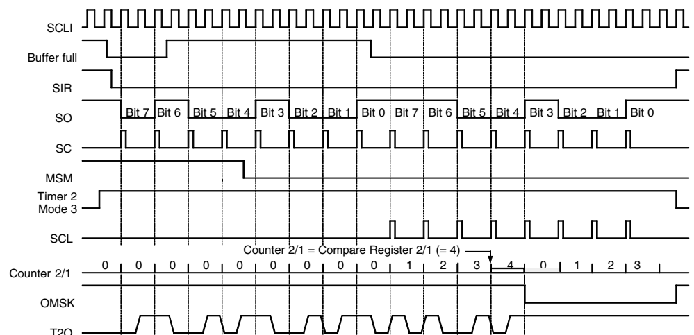
Figure 72. Manchester Modulation 2
