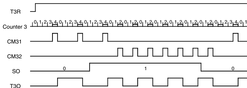
Figure 85. FSK Modulation
