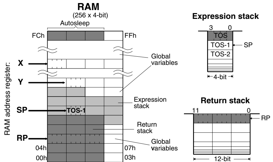
Figure 5. RAM Map
