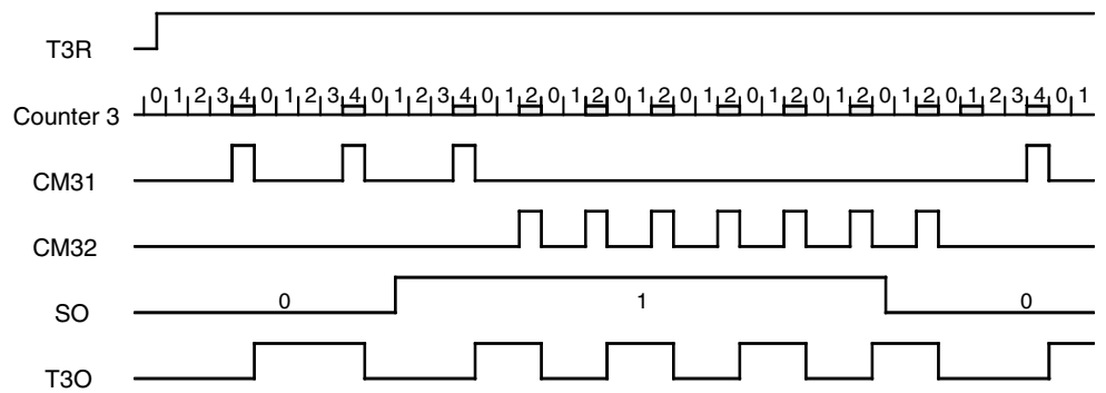
Figure 51. FSK Modulation
