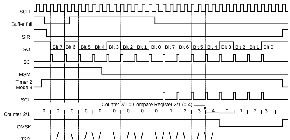
Figure 78. Manchester Modulation 2
