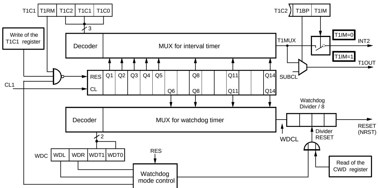
Figure 35. Timer 1 and Watchdog
