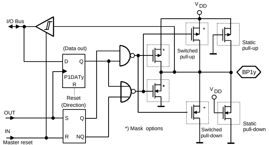
Figure 28. Bi-directional Port 1
