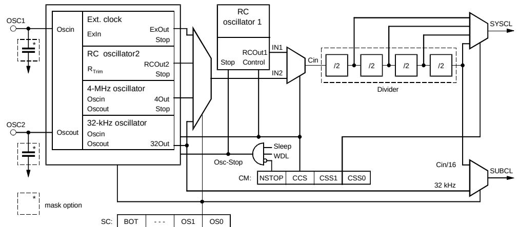
Figure 21. Clock Module
