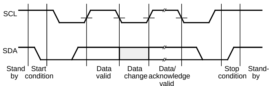
Figure 94. MCL Protocol
