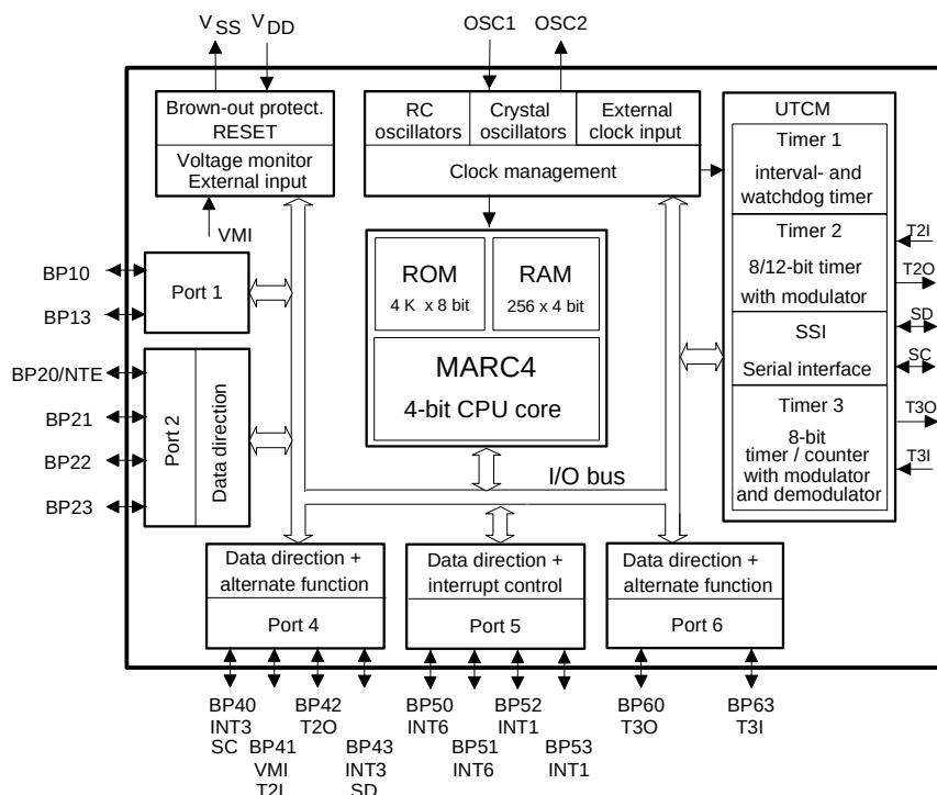
Figure 9. Block Diagram
