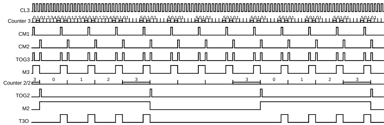
Figure 88. Burst Modulation 1
