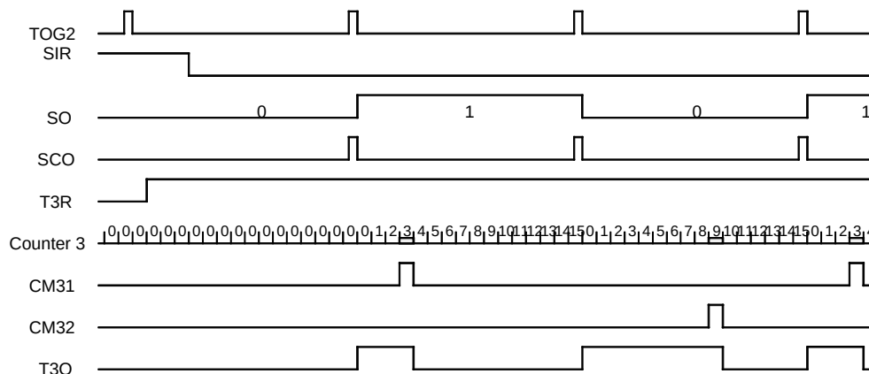
Figure 58. Pulse-width Modulation
