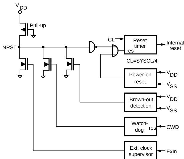
Figure 16. Reset Configuration
