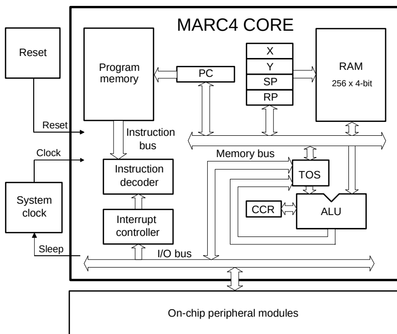
Figure 10. MARC4 Core
