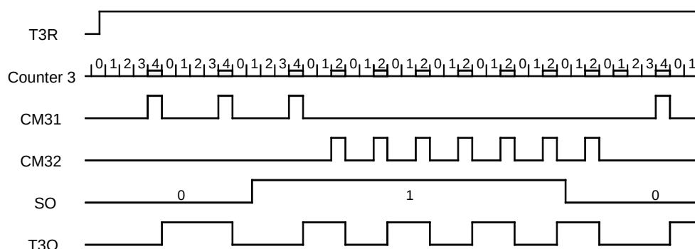
Figure 91. FSK Modulation
