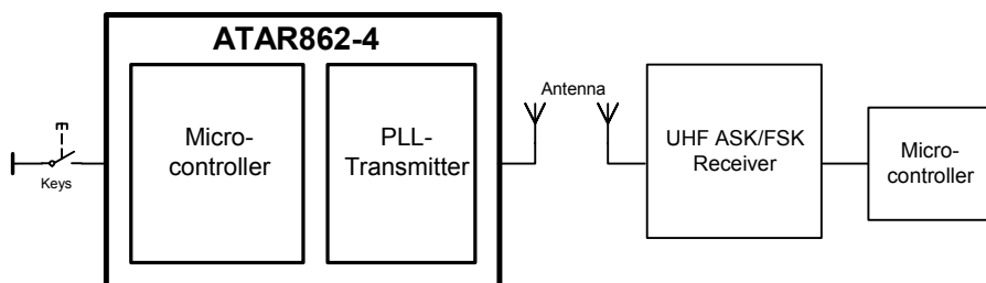
Figure 1. Application Diagram
