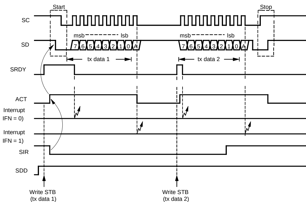
Figure 68. Example of MCL Transmit Dialog
