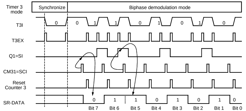
Figure 84. Biphase Demodulation
