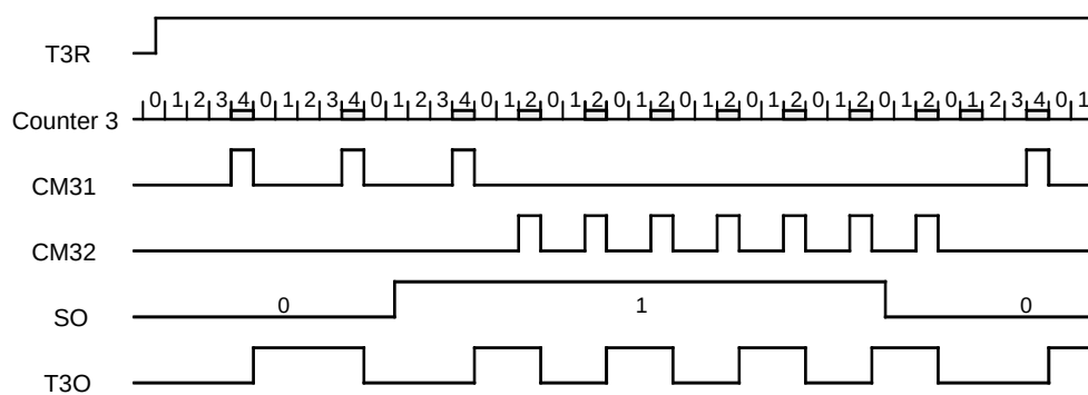
Figure 57. FSK Modulation
