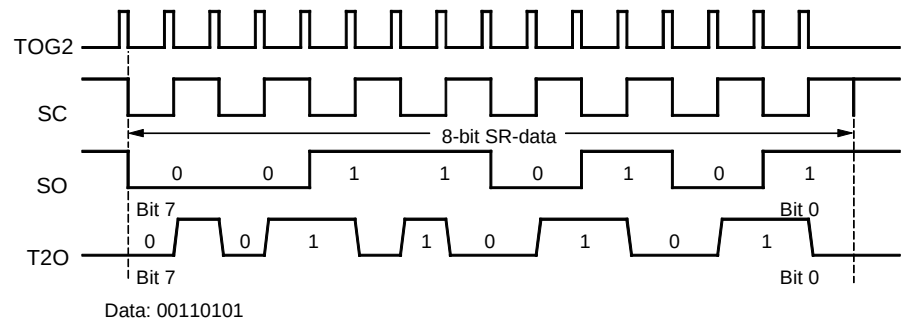
Figure 77. Manchester Modulation 1
