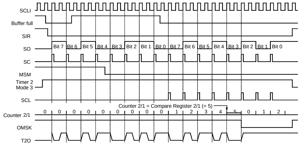
Figure 79. Biphase Modulation
