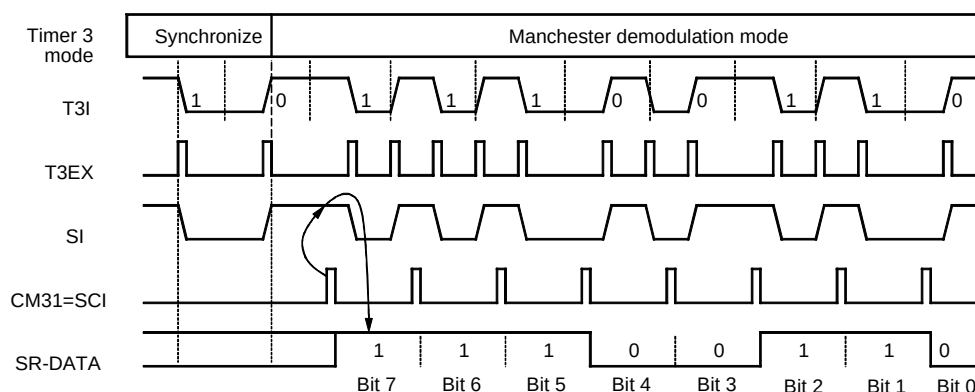
Figure 83. Manchester Demodulation
