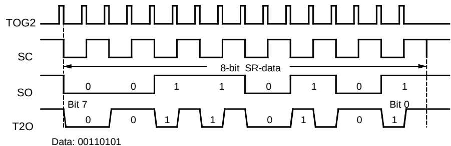
Figure 76. Biphase Modulation 1
