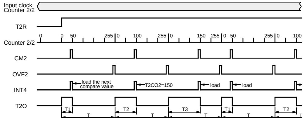
Figure 48. PWM Modulation
