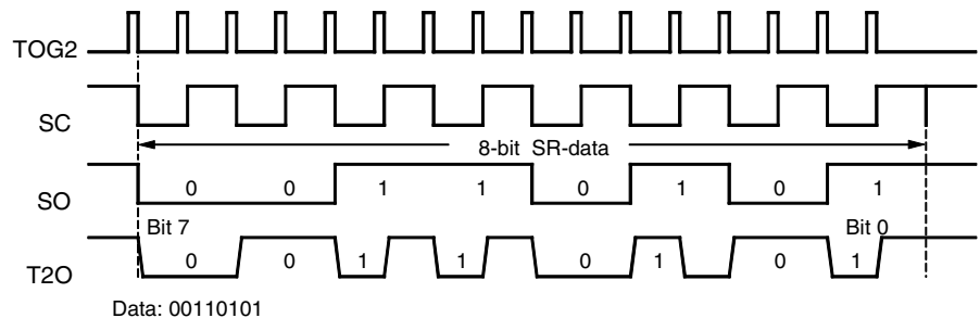
Figure 70. Biphase Modulation 1
