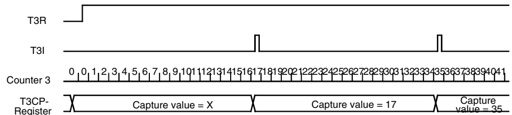
Figure 55. External Capture Mode
