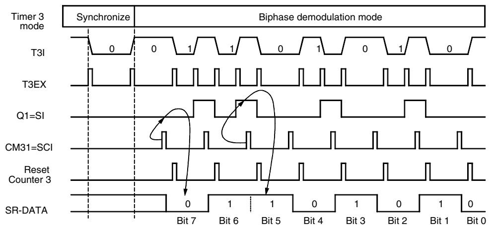
Figure 78. Biphase Demodulation
