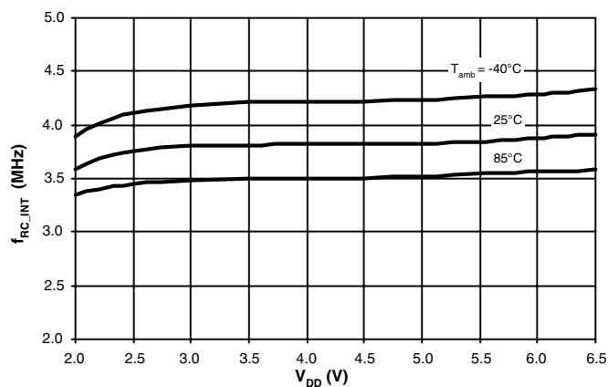
Figure 96. Internal RC Frequency versus V_{DD}
