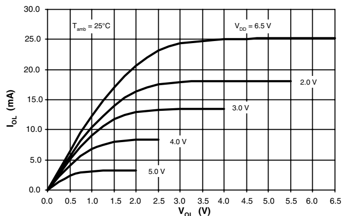
Figure 107. Output Low Current versus Output Low Voltage
