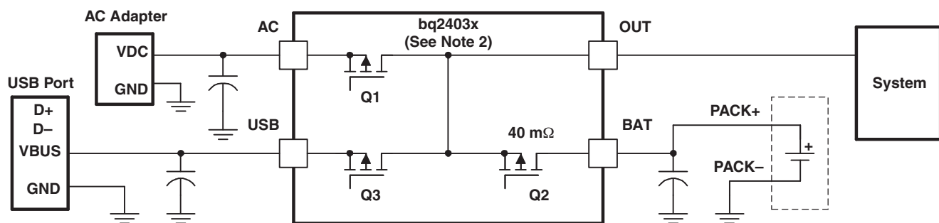
Figure 4. Power-Path Management
