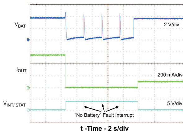
Figure 4. Battery Insertion/Removal
