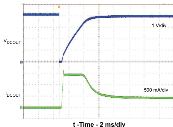
Figure 17. Hotplug 1000μF Capacitor into DCOUT
