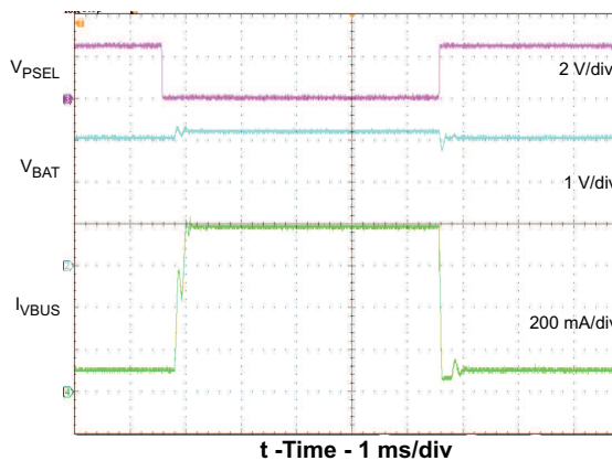
Figure 14. PSEL Transition
