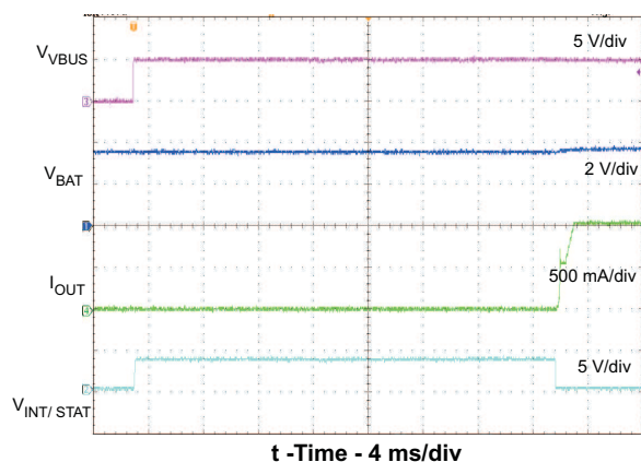
Figure 3. Adapter Insertion
