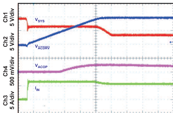
SELECTOR GATE DRIVE VOLTAGES, 700 MS DELAY AFTER ACDET
