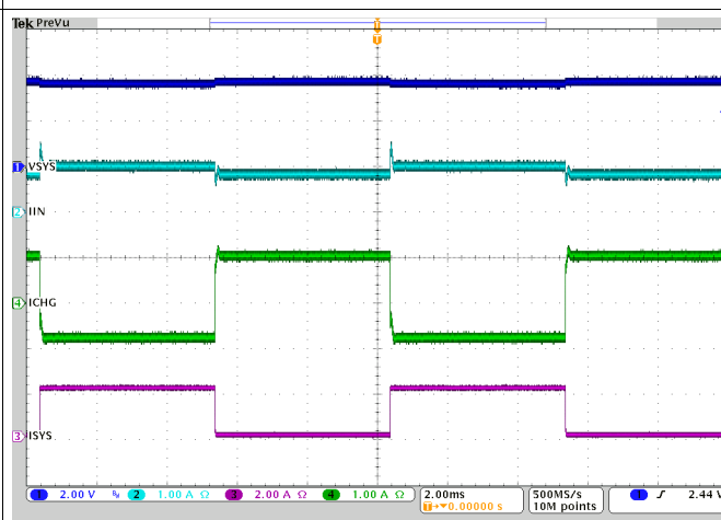
Figure 28. OTG Switching
