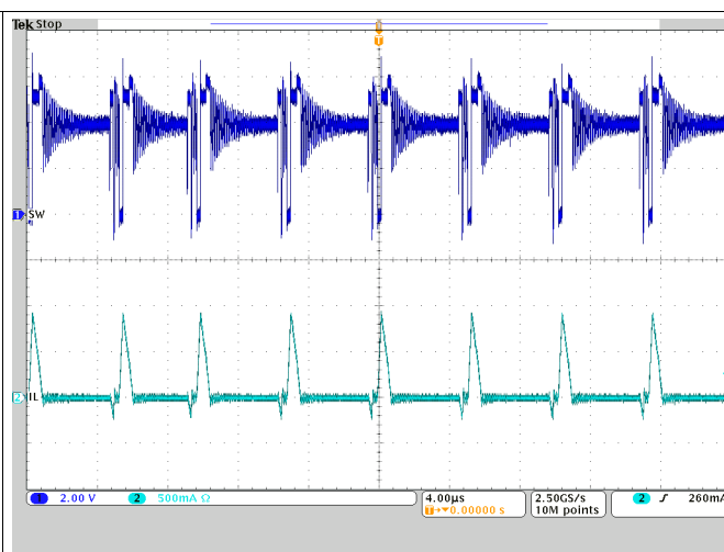
Figure 28. OTG Switching
