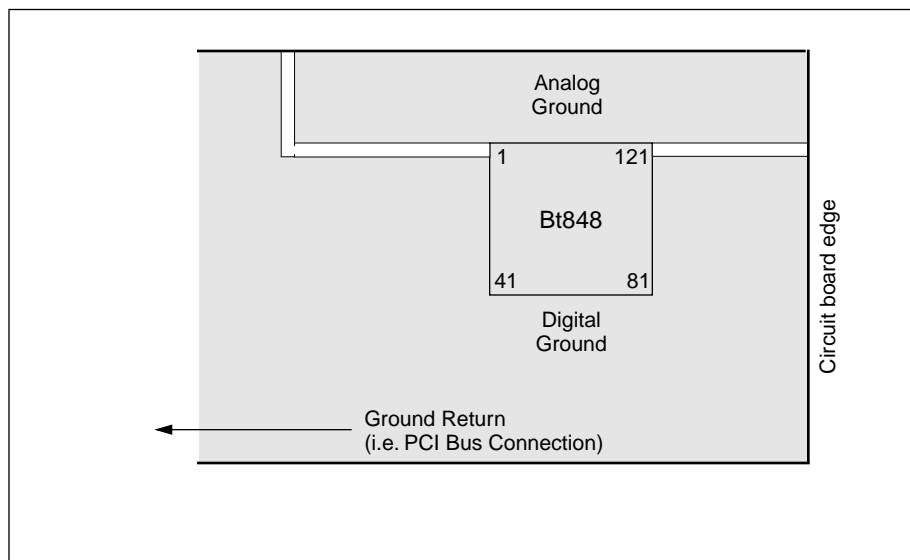
Figure 35. Example Ground Plane Layout
