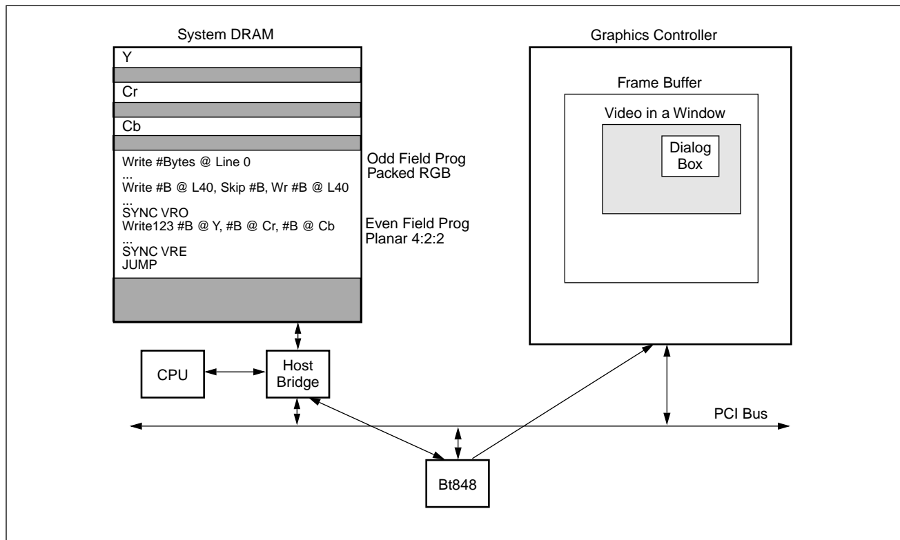
Figure 22. Example of Bt848 Performing Complex Clipping
