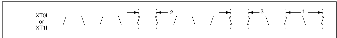
Figure 39. Clock Timing Diagram
