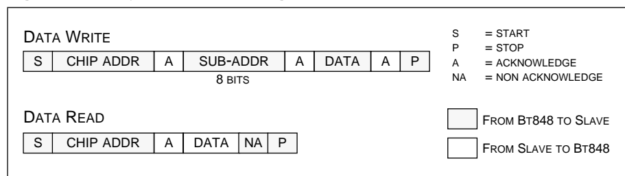
Figure 33. I 2 C Typical Protocol Diagram
