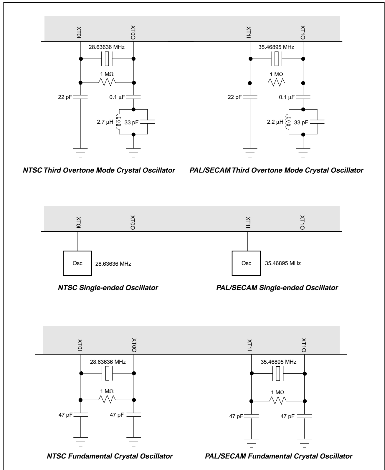
Figure 24. Clock Options
