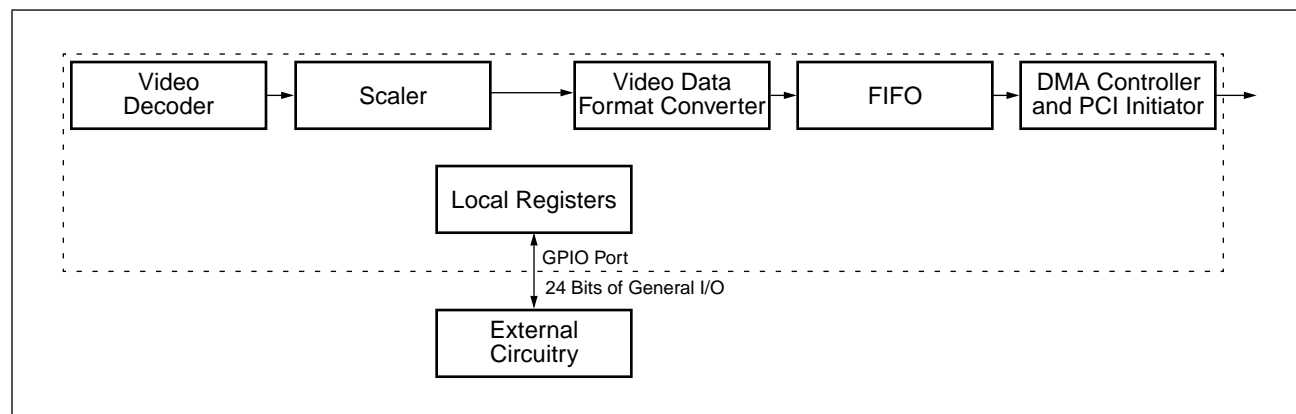
Figure 27. GPIO Normal Mode
