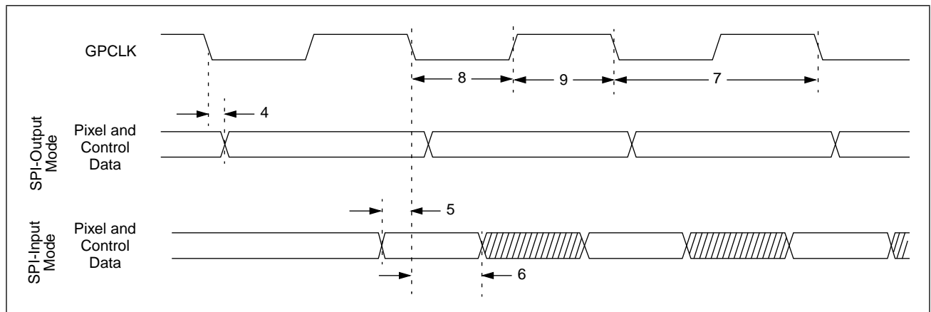
Figure 40. GPIO Timing Diagram
