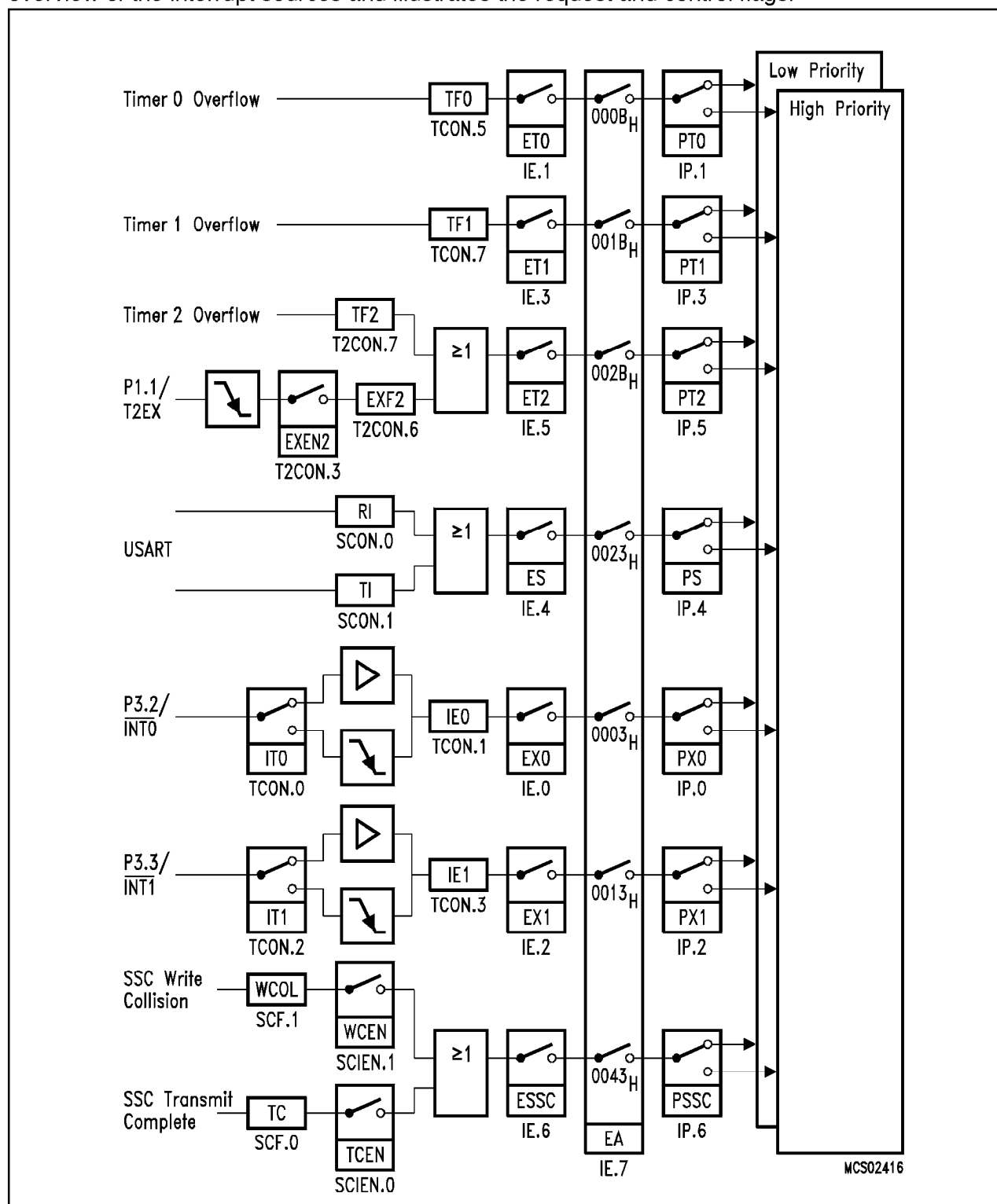
Figure 10 Interrupt Request Sources
