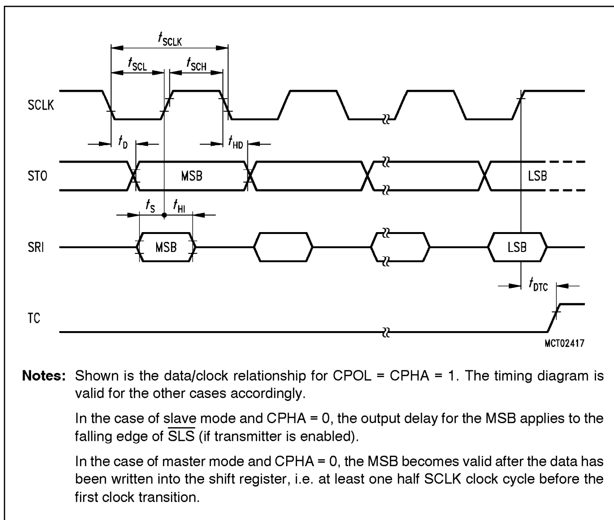
Figure 14 SSC Timing
