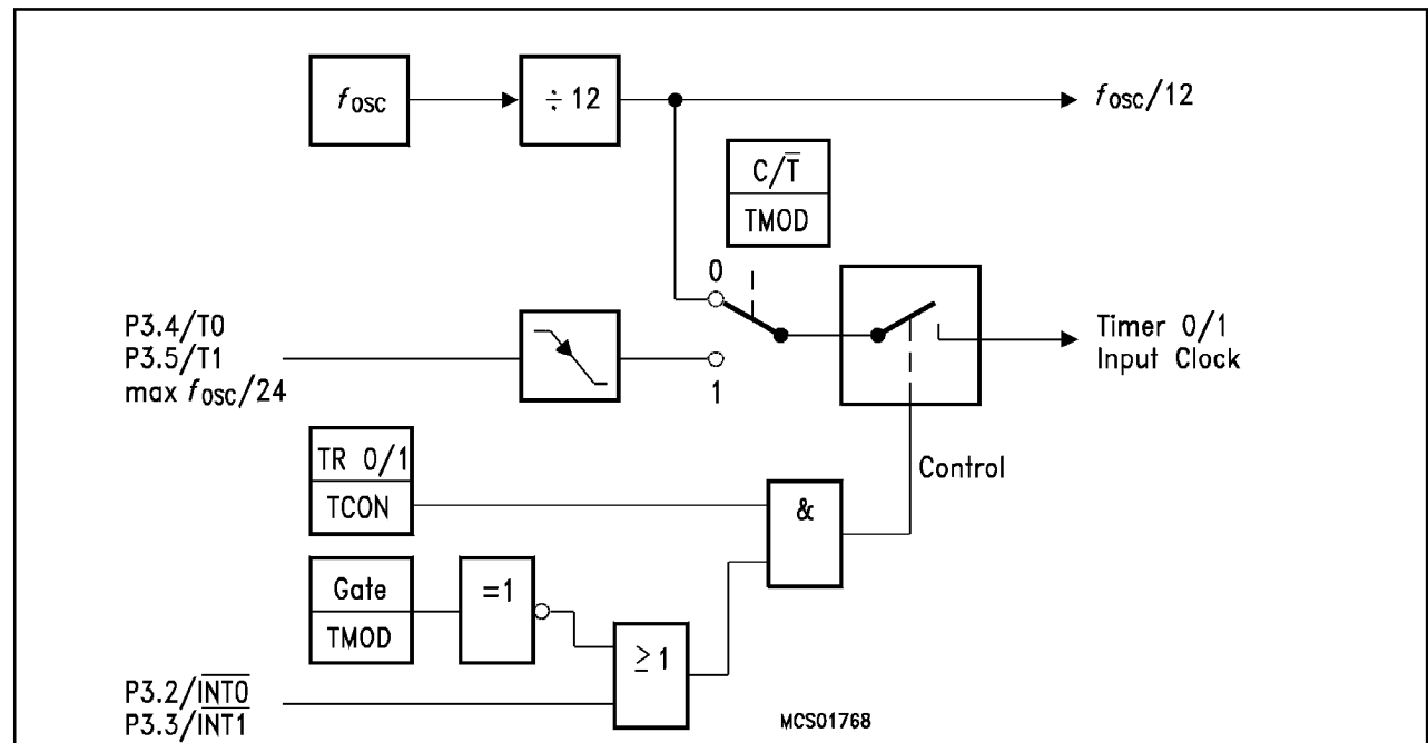
Figure 7 Timer/Counter 0 and 1 Input Clock Logic
