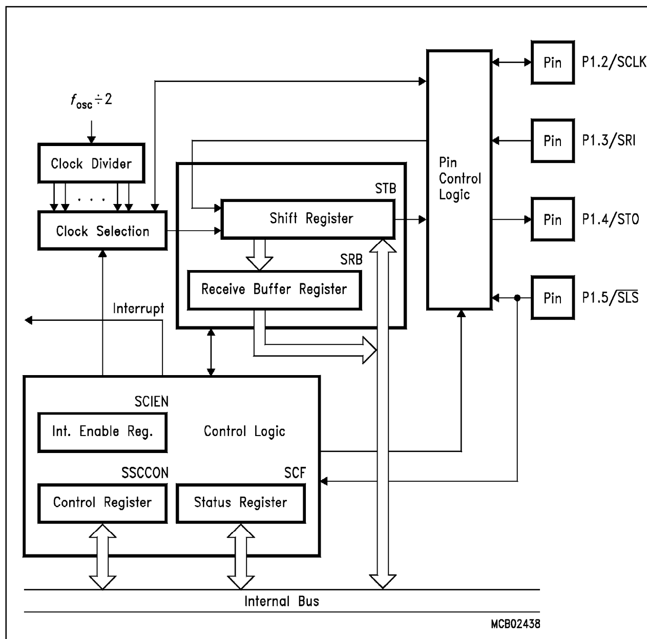
Figure 9 SSC Blockdiagram
