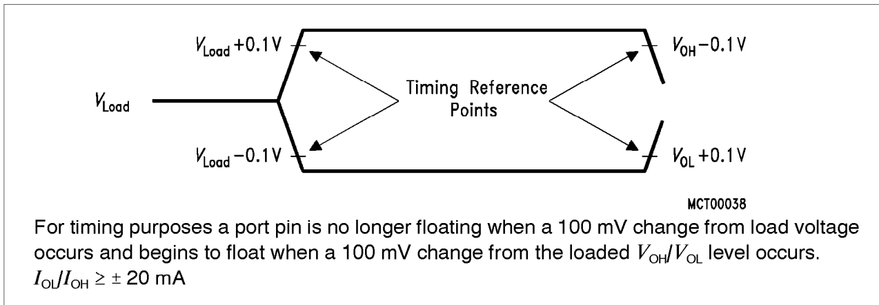
Figure 21 AC Testing: Float Waveforms
