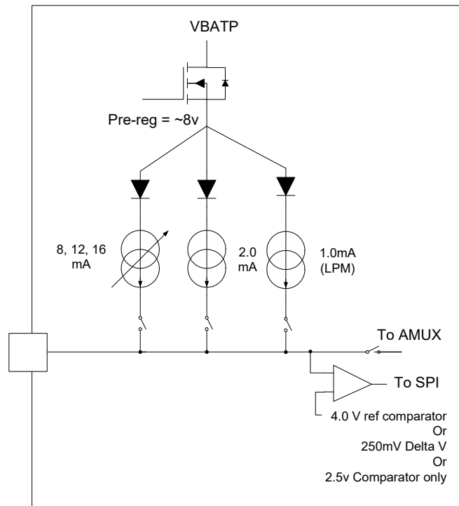
Figure 15. SG block diagram
