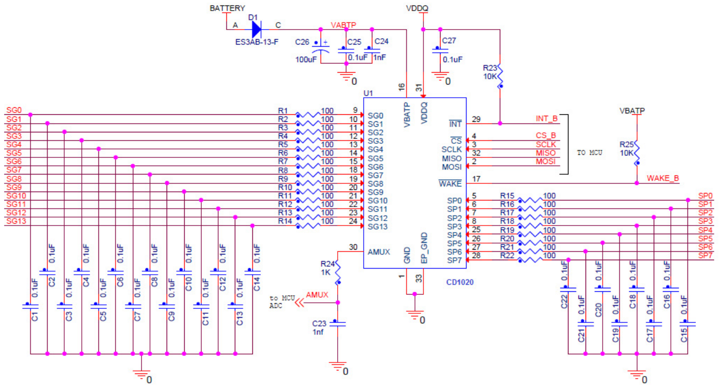
Figure 22. Typical application diagram
